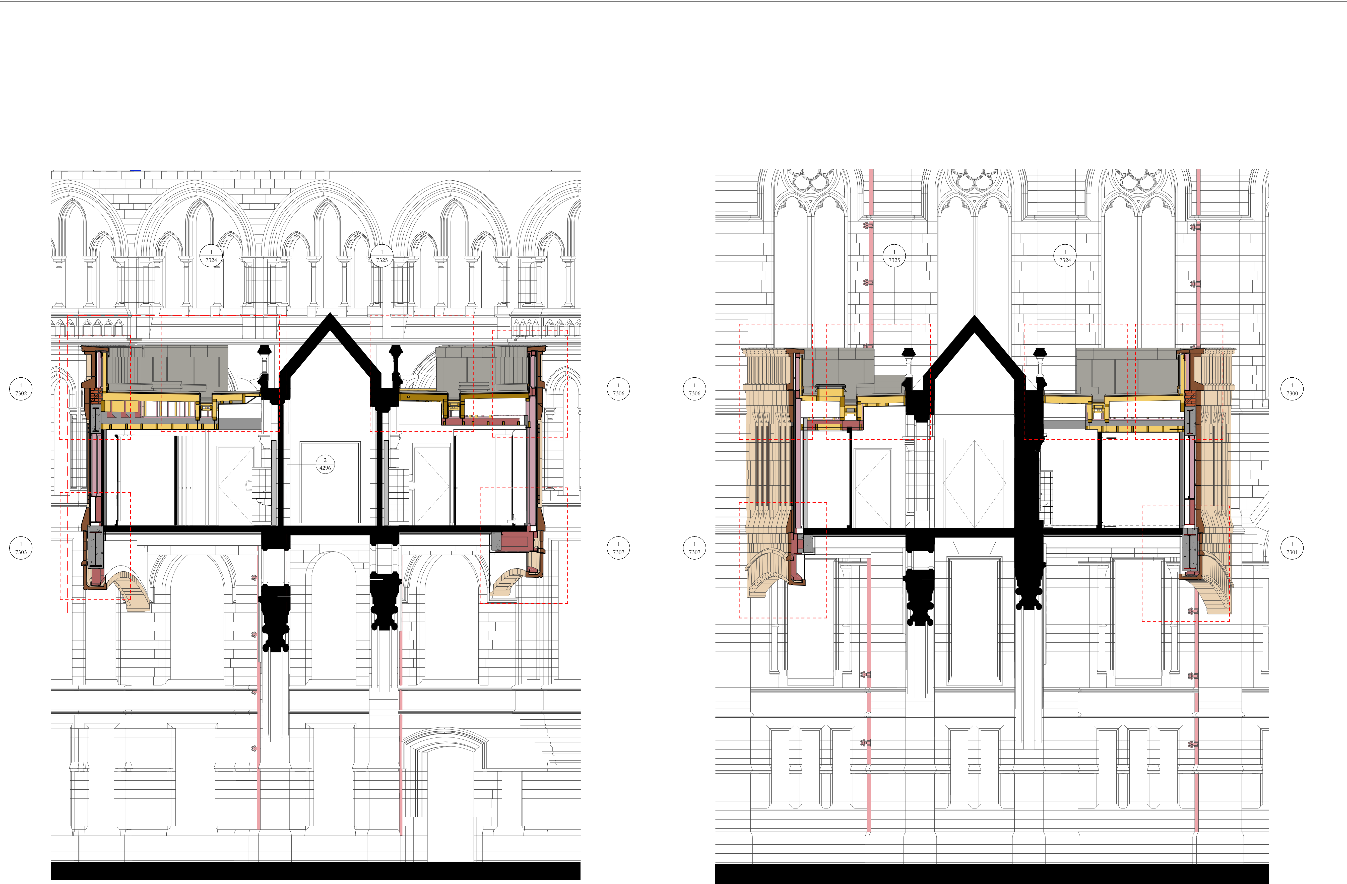
Link Bridge Section AA 1 : 50
