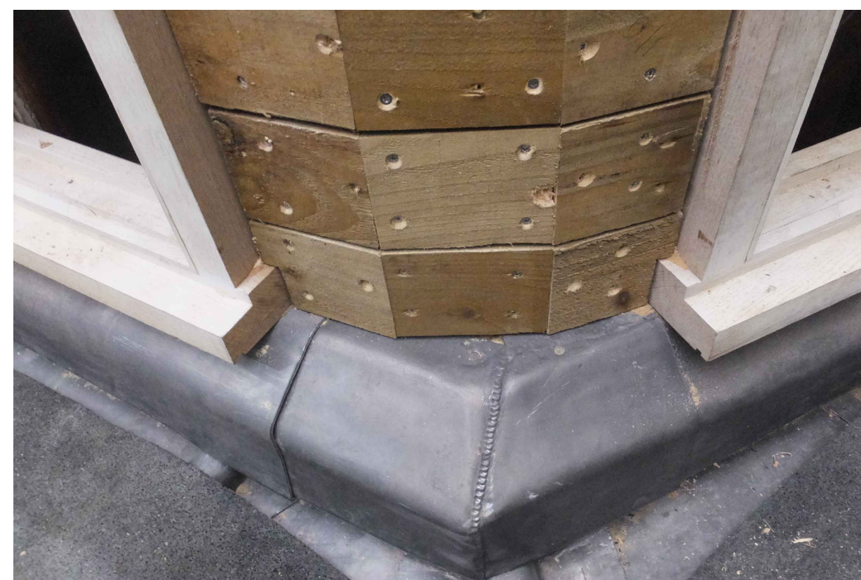
EXISTING CILL DETAIL AT CORNER OF ROOF LIGHT
