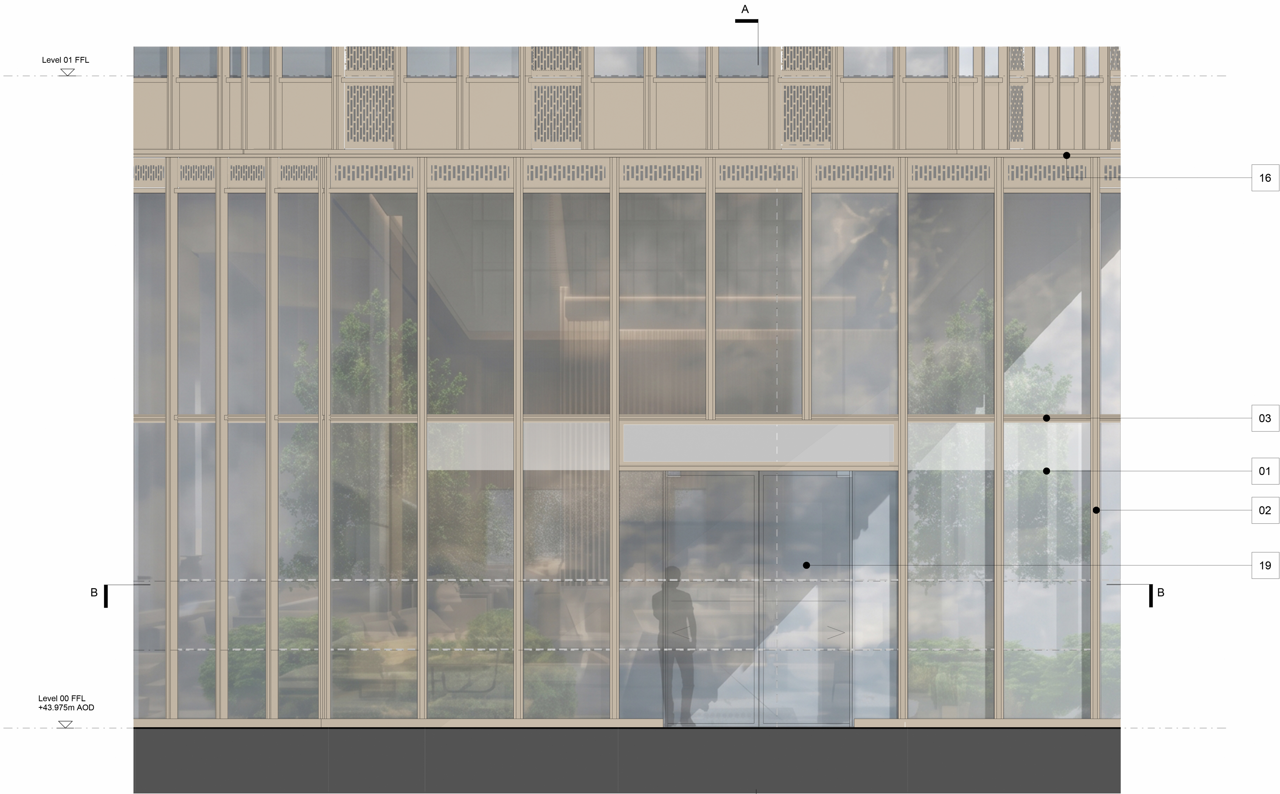
Detail Elevation 1:25
