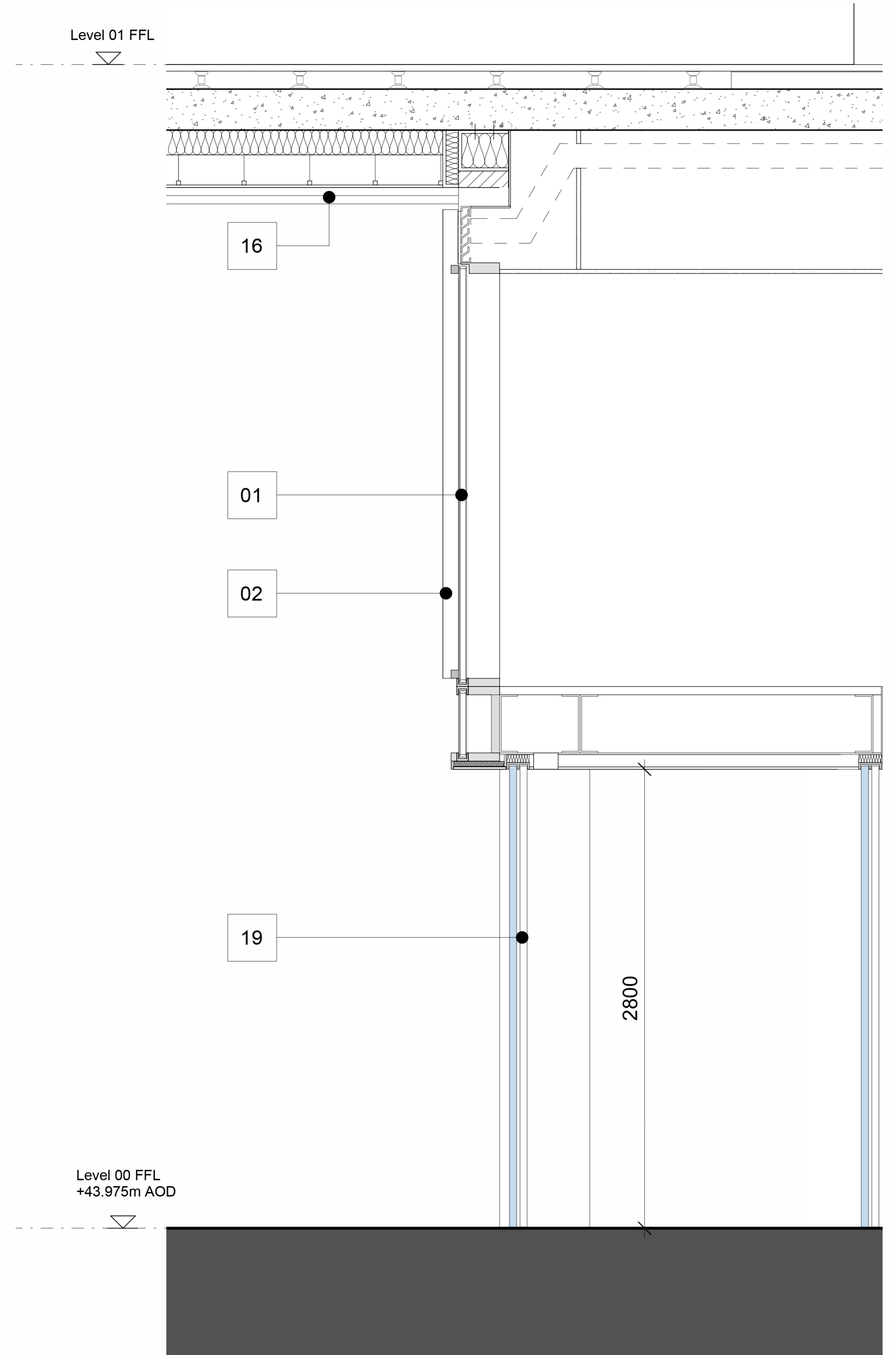
Detail Section AA 1:25
