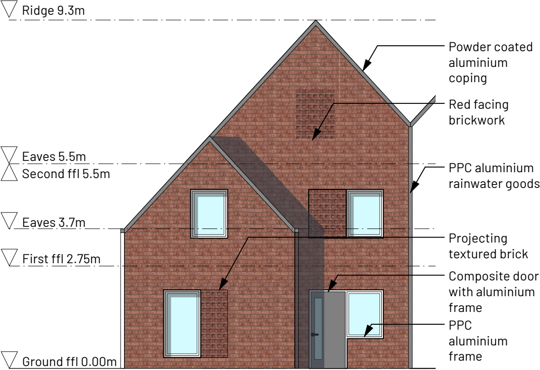
1 Front Elevation (Type C) Scale: 1:100
