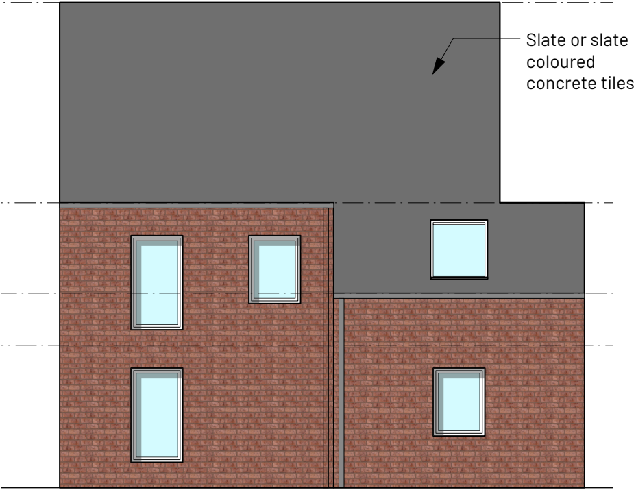
2 Side Elevation (Type C) Scale: 1:100
