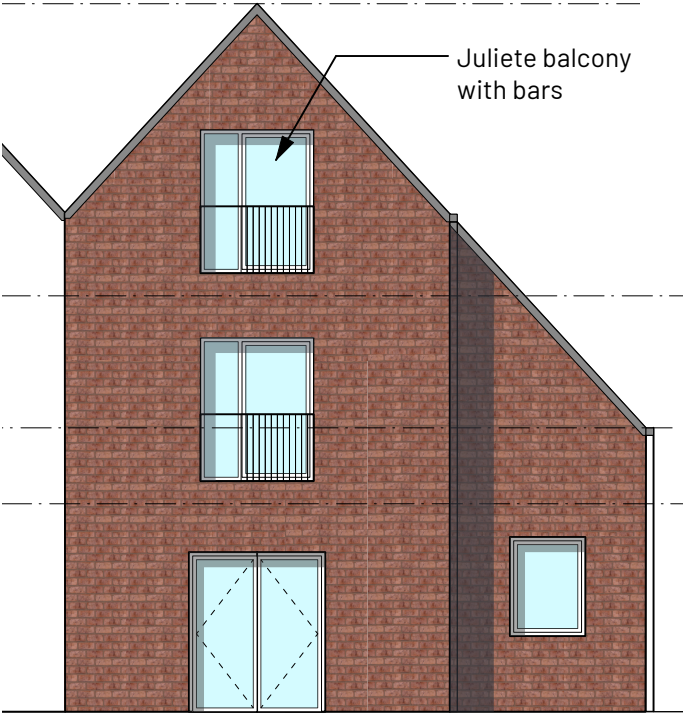
3 Rear Elevation (Type C) Scale: 1:100
