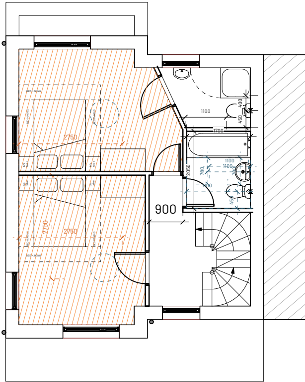
2 Ground Floor Plan Scale: 1:100
