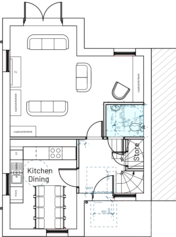
1 Ground Floor Plan Scale: 1:100
