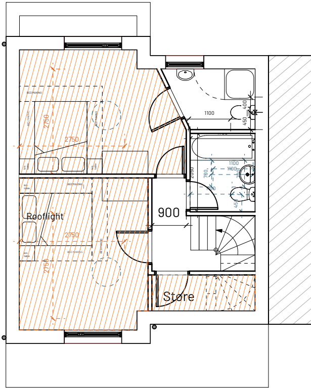
3 Ground Floor Plan Scale: 1:100
