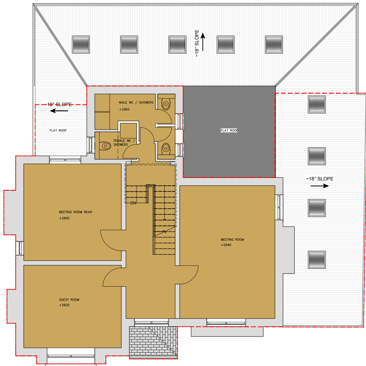
Proposed First Floor/ Lower Roof Plan 1 : 100
