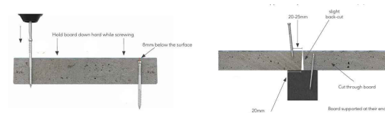
Millboard Score Fixing Details
