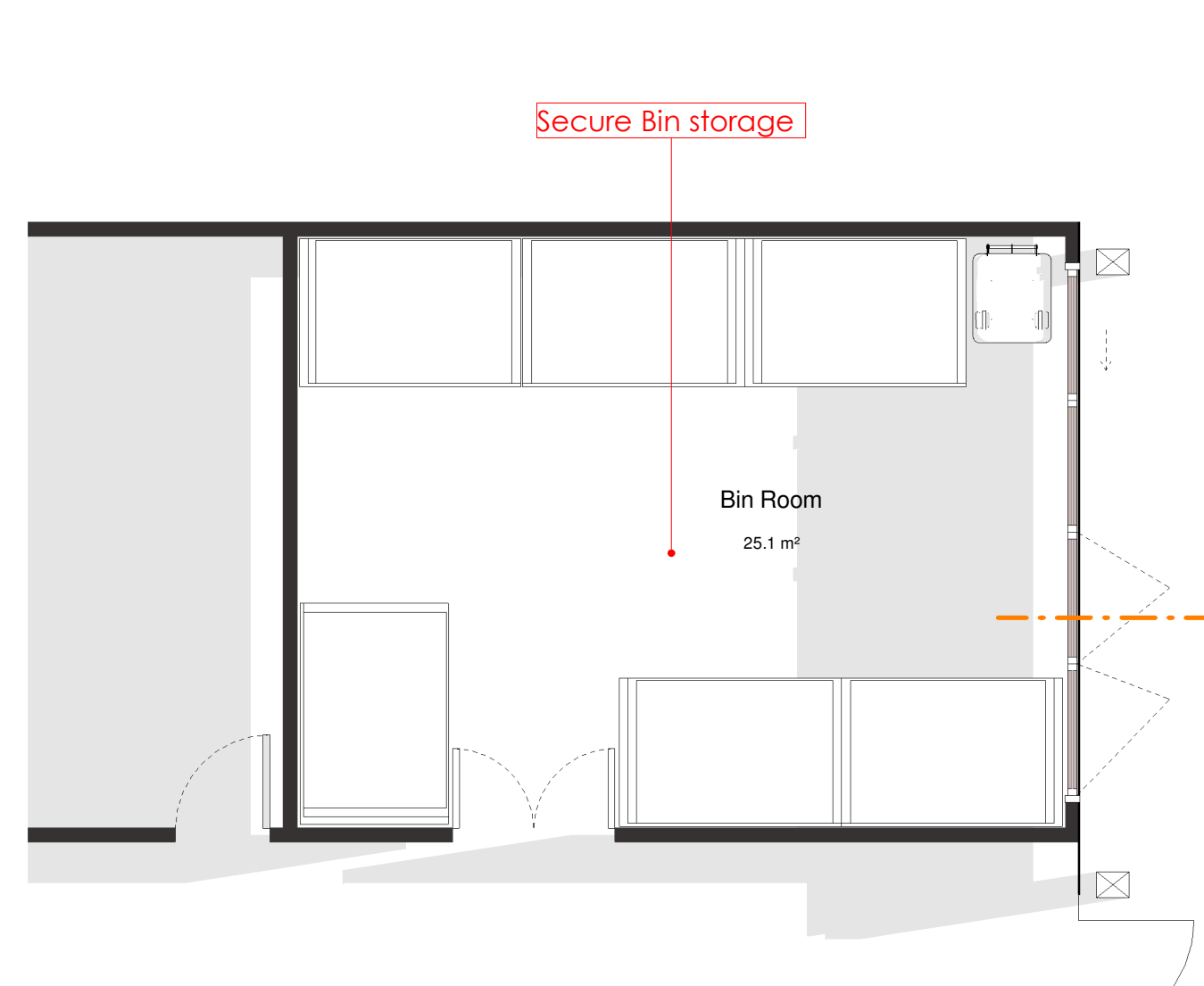
2 Bin Store Plan 1 : 50
