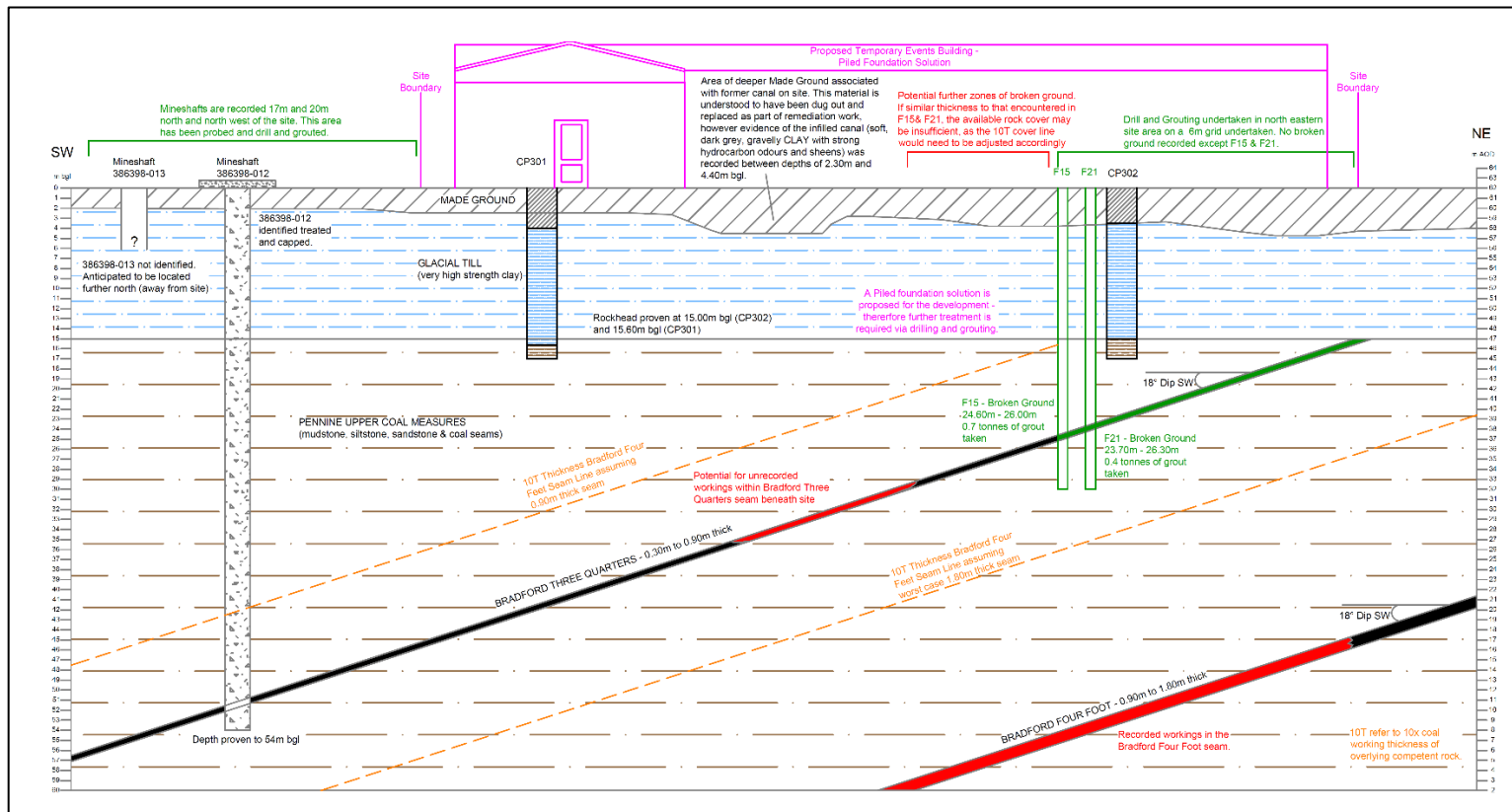
Figure 8: Extract of the conceptual ground model for the site.
