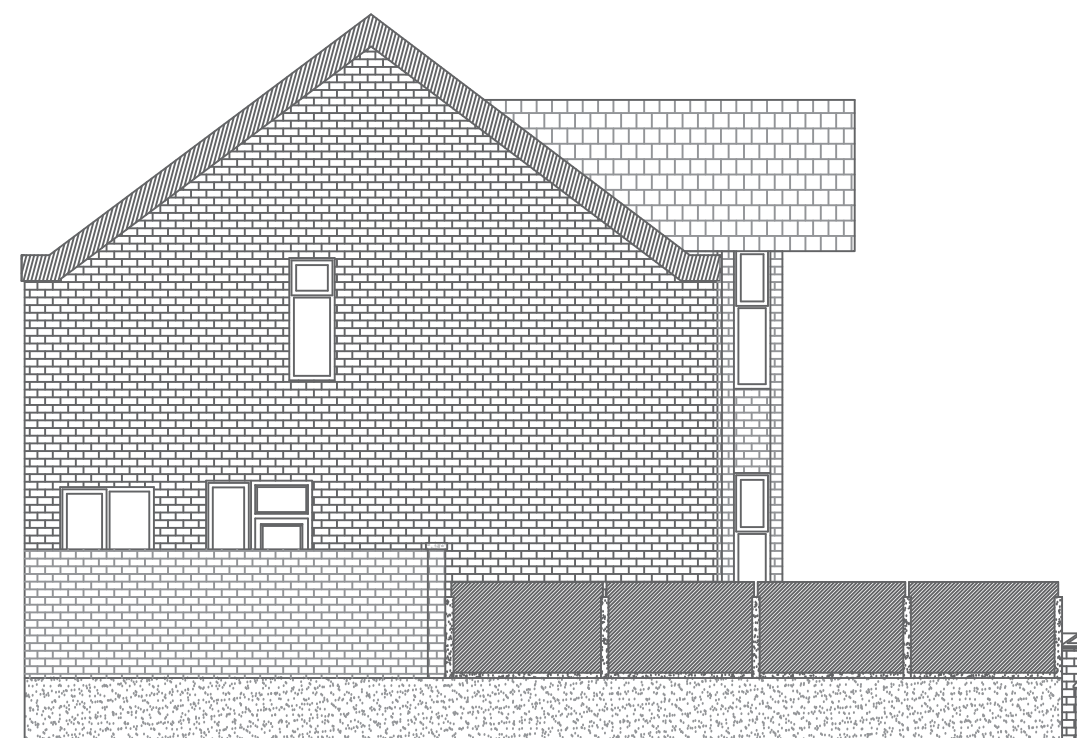
Existing L/H/S Elevation
