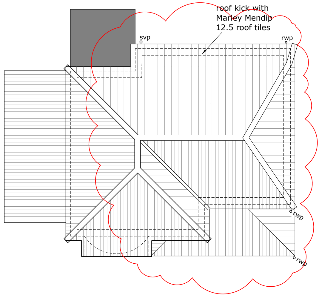
ROOF PLAN
