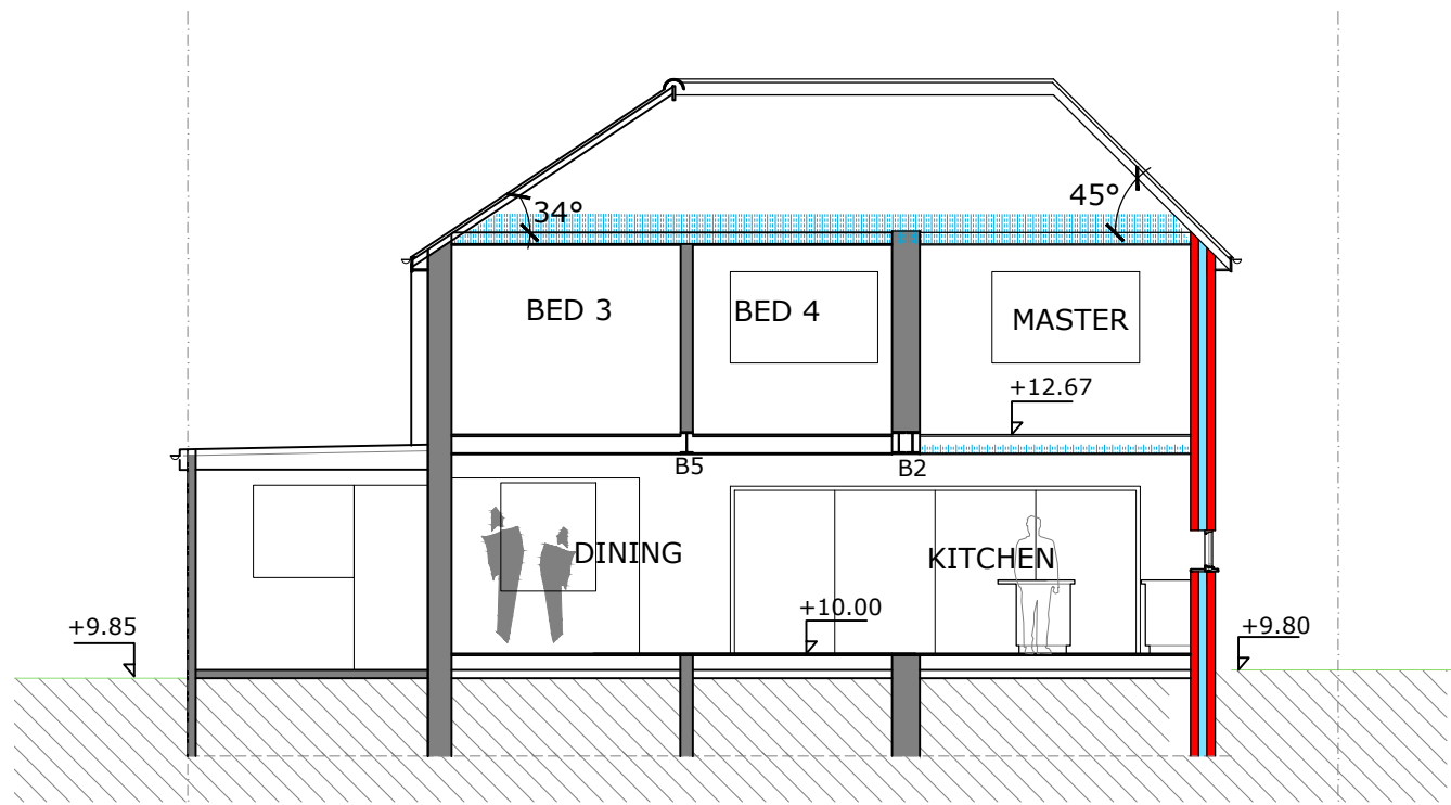
CROSS SECTION
