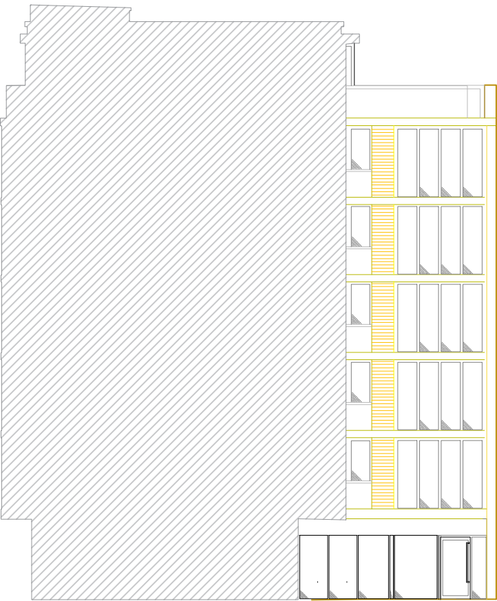
Worsley Street Elevation
