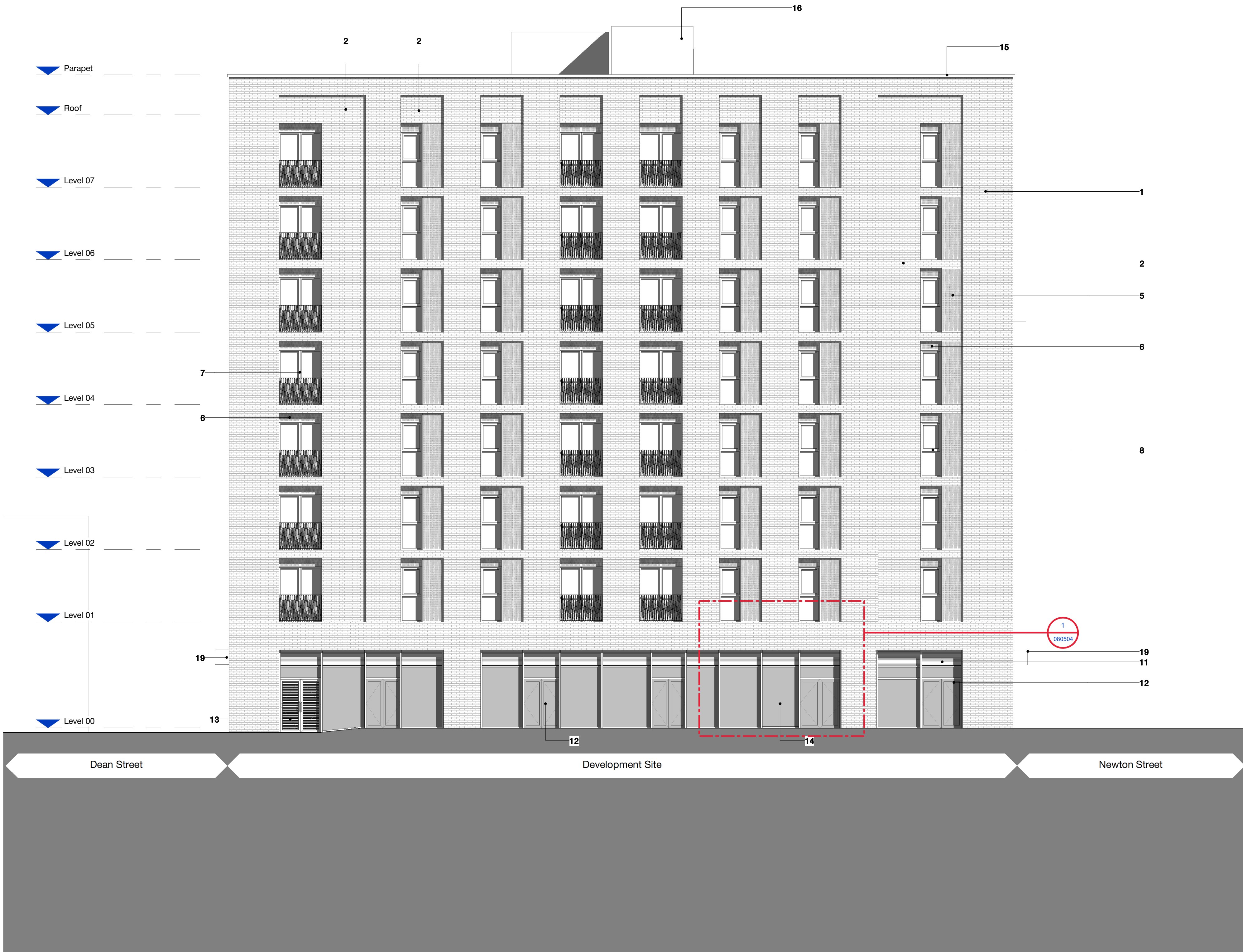
Proposed Postal Street Elevation 1 : 100
