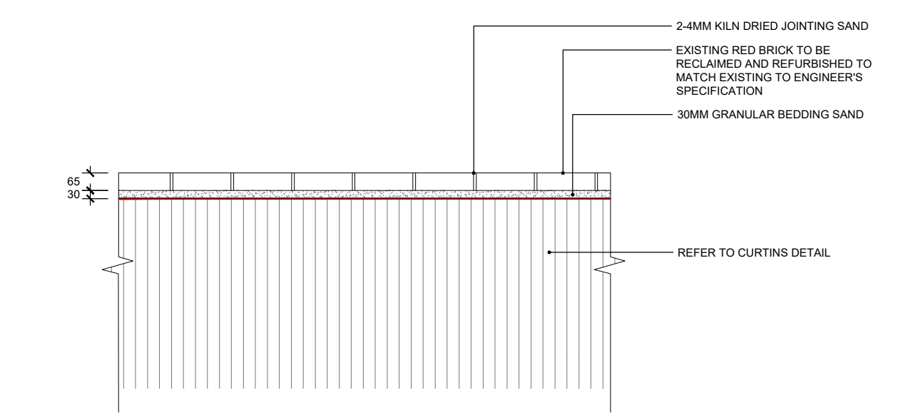
06A 00600 RECLAIMED RED BRICK SECTION
