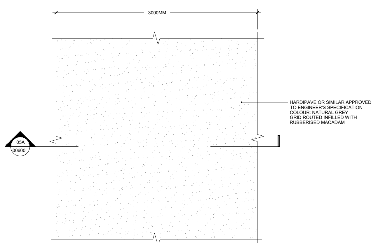
05B 00600 HARDPAVE PLAN
