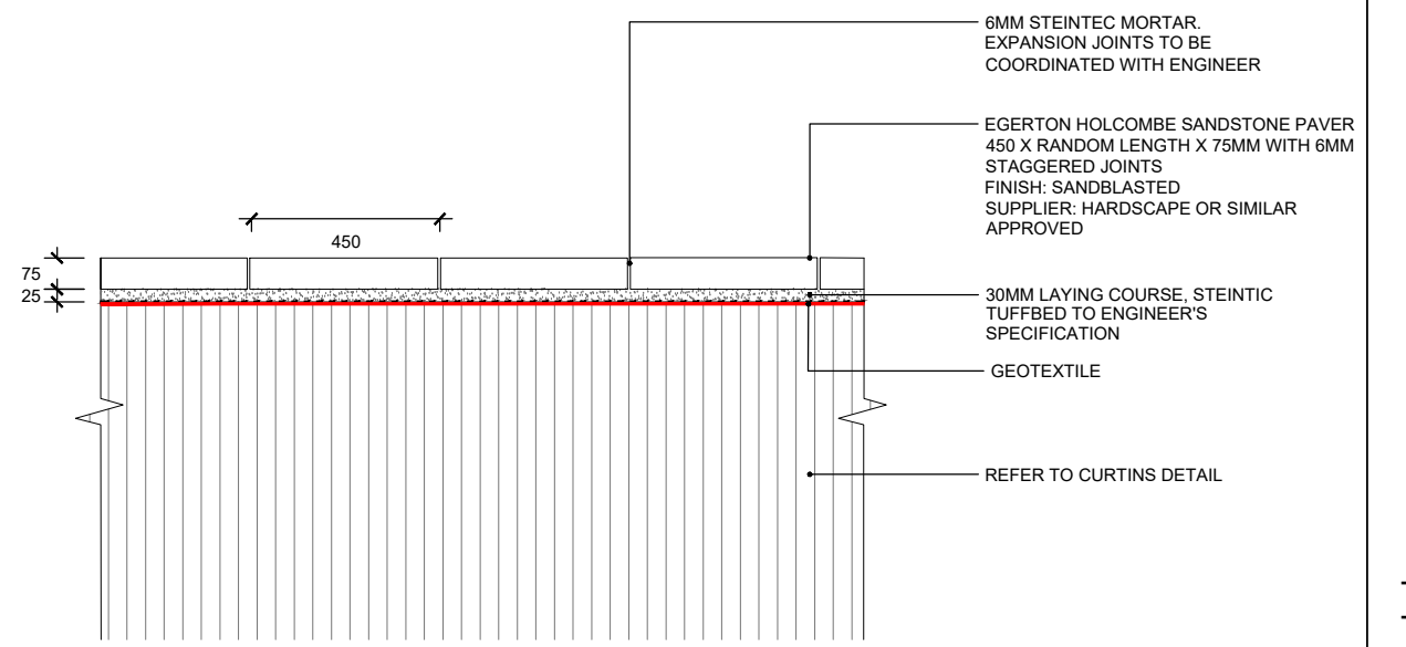
08A 00600 SANDSTONE PAVING SECTION
