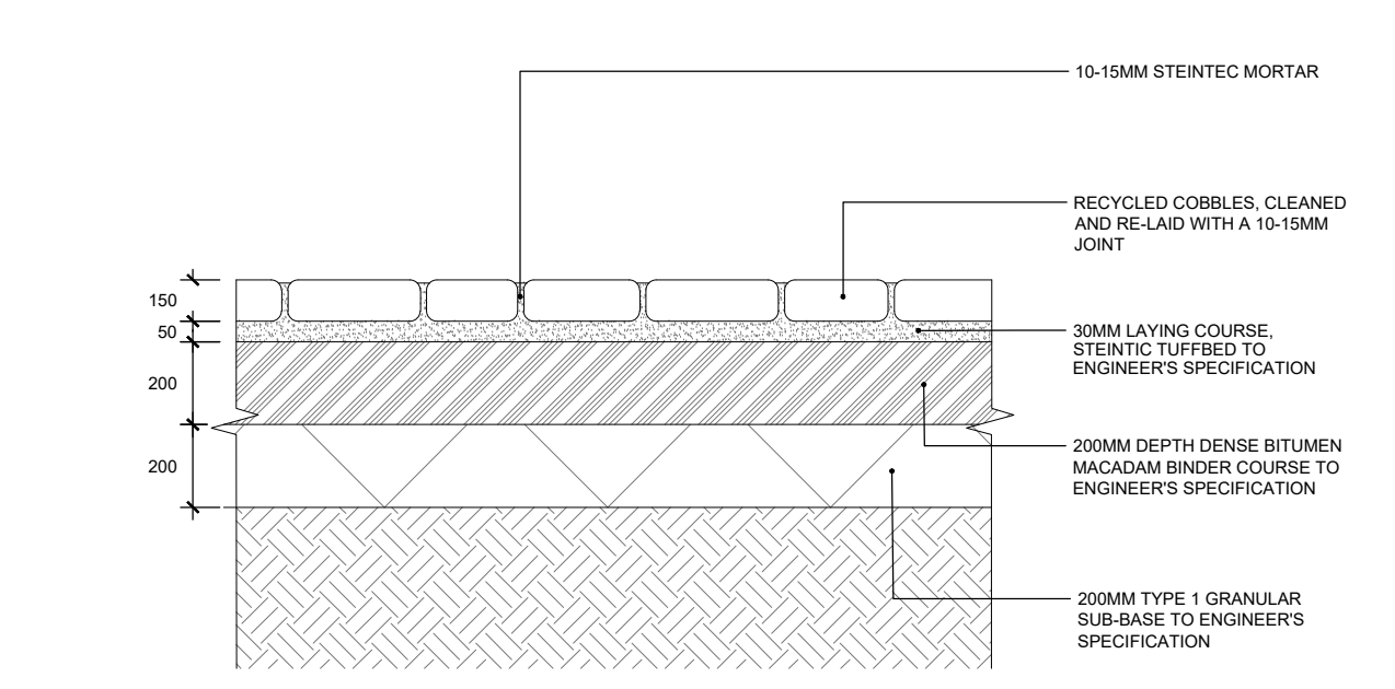
03A 00600 RECLAIMED COBBLES SECTION
