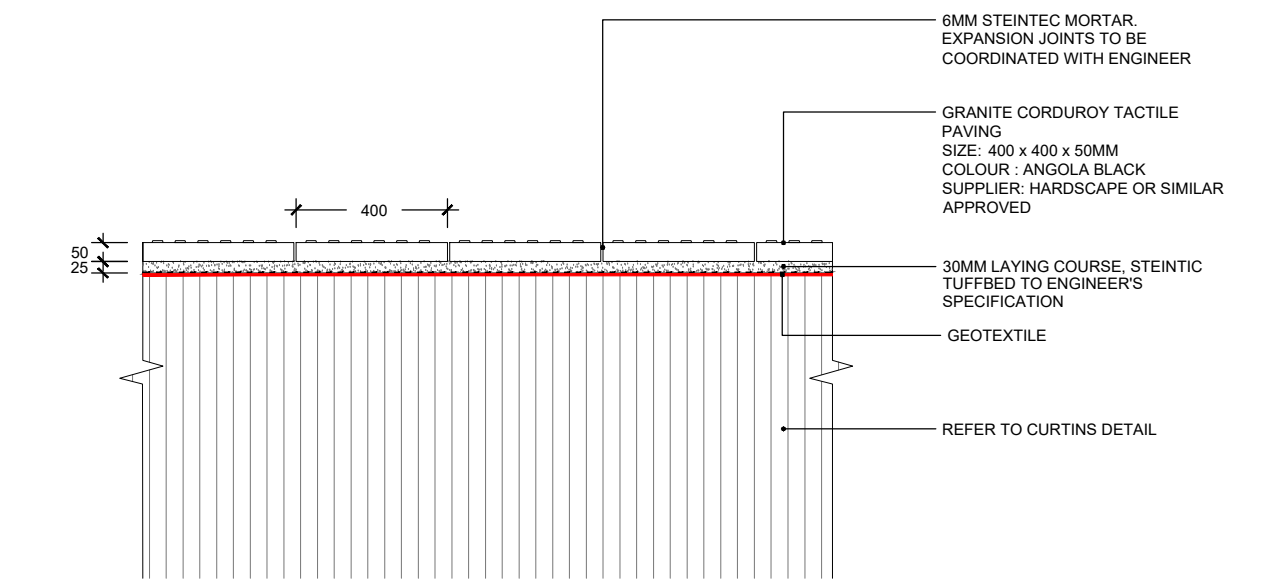
07A 00600 CORDUROY GRANITE PAVING SECTION
