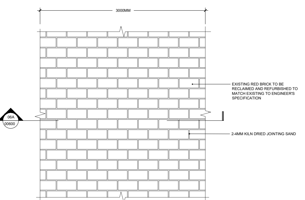
06B 00600 RECLAIMED RED BRICK PLAN
