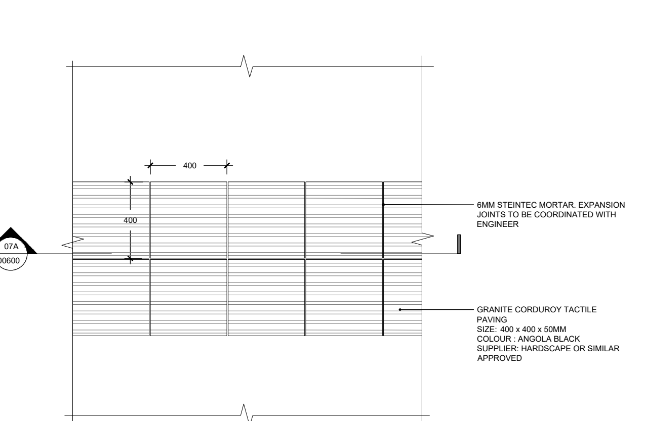
07B 00600 CORDUROY GRANITE PAVING PLAN
