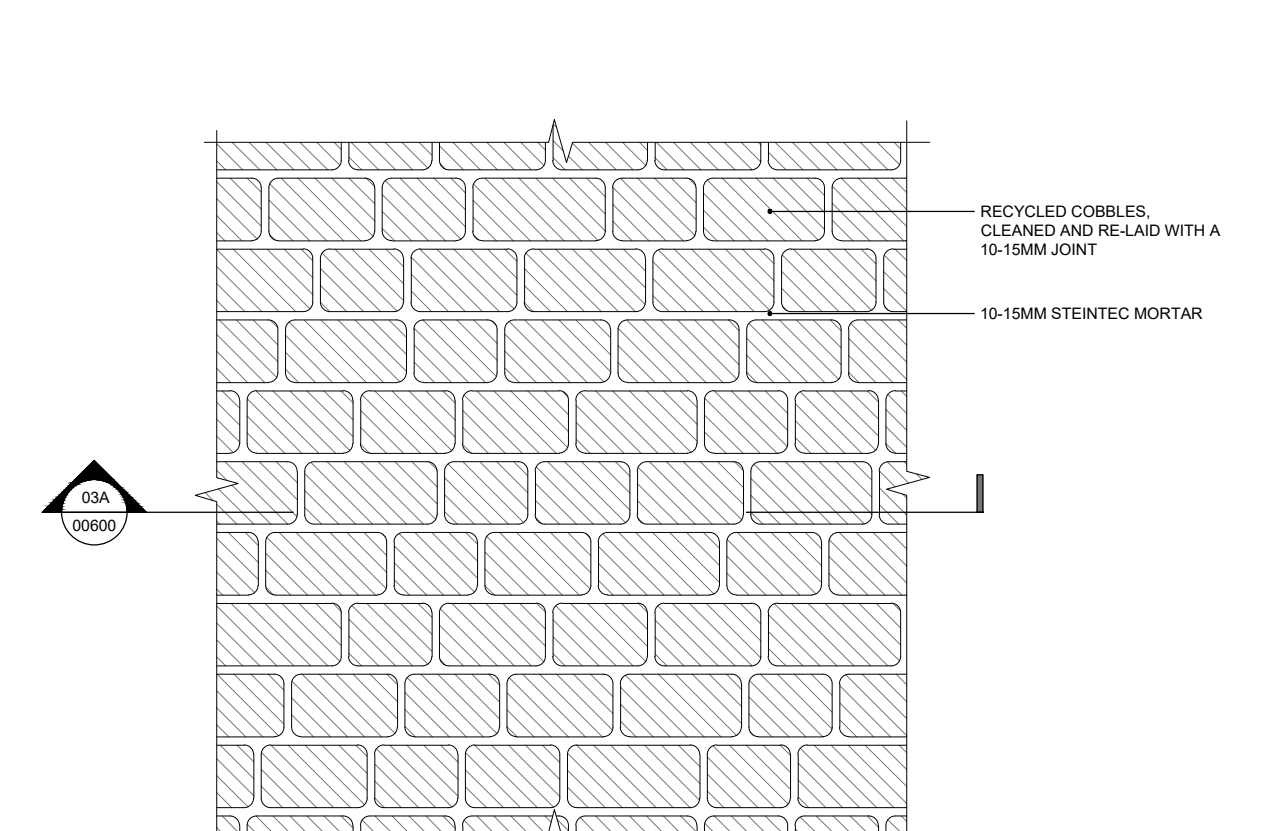
03B 00600 RECLAIMED COBBLES PLAN
