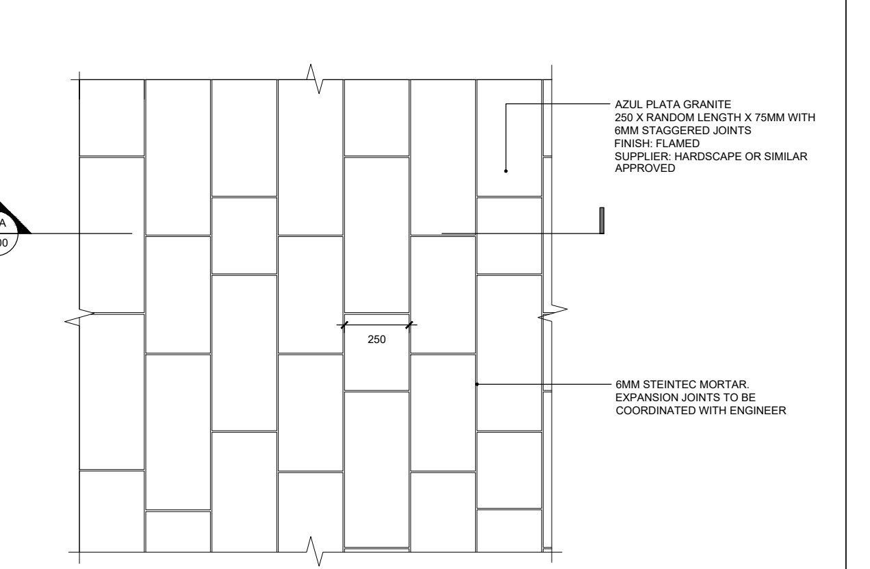
04B 00600 GRANITE STONE PAVING PLAN
