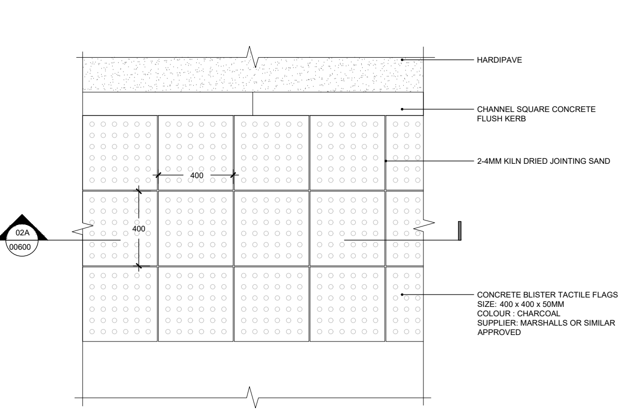
02B 00600 BLISTER CONCRETE PAVING PLAN
