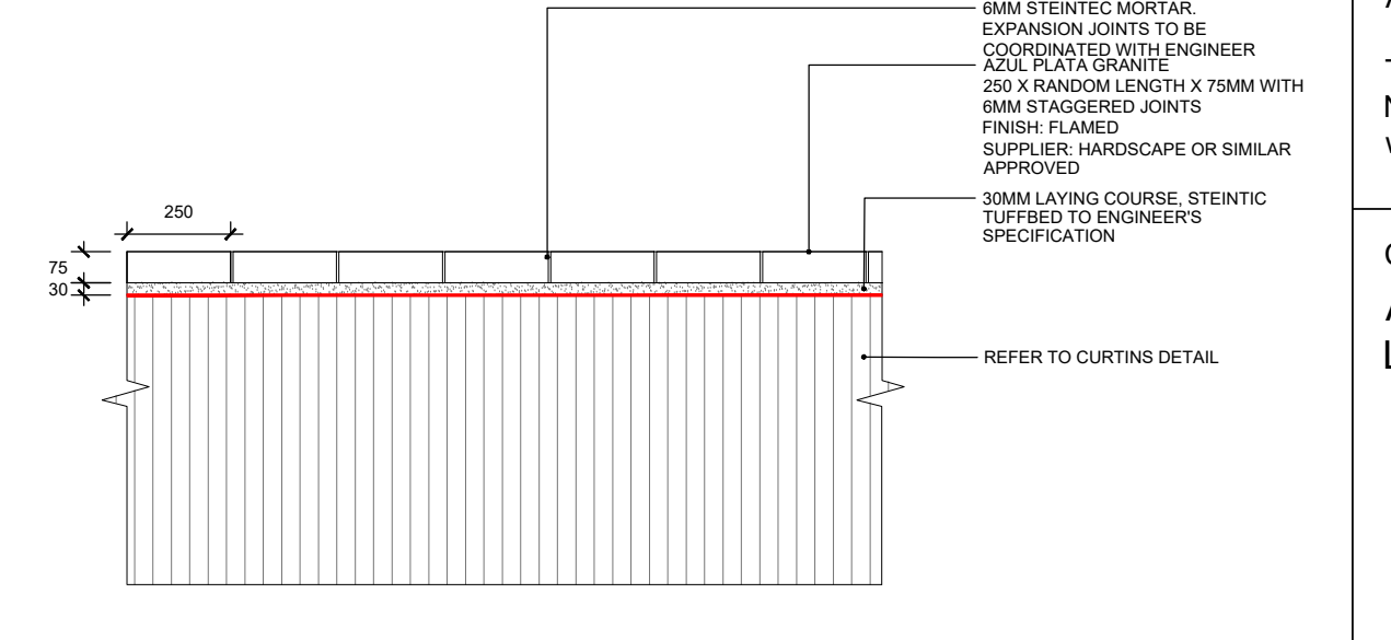
04A 00600 GRANITE STONE PAVING SECTION
