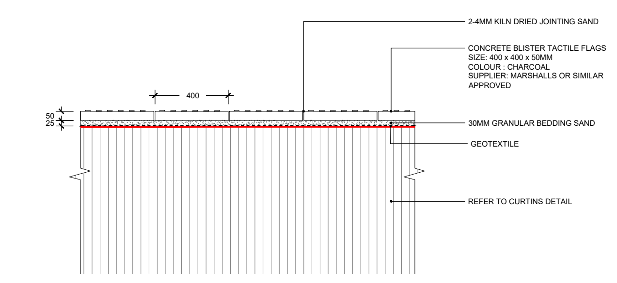
02A 00600 BLISTER CONCRETE PAVING SECTION
