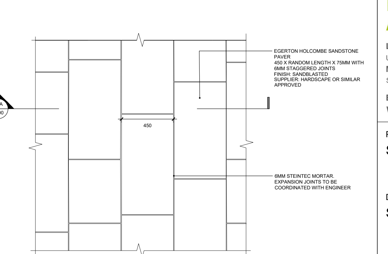
08B 00600 SANDSTONE PAVING PLAN
