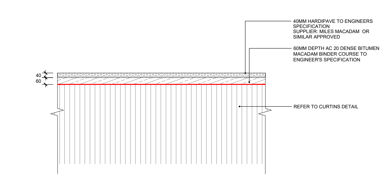
05A 00600 HARDPAVE SECTION
