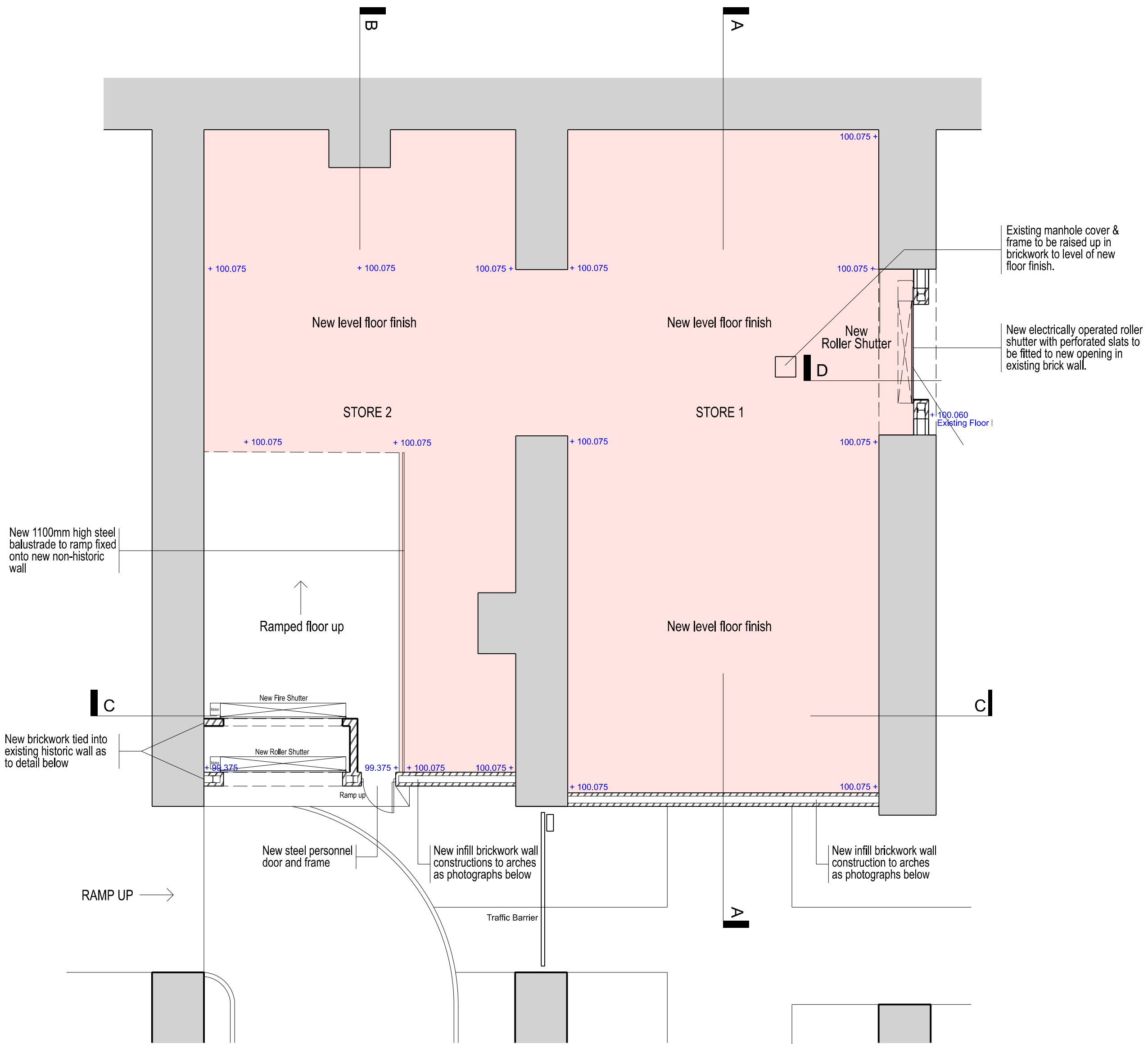
PROPOSED FLOOR PLAN OF NEW STORAGE AREA 1:100
