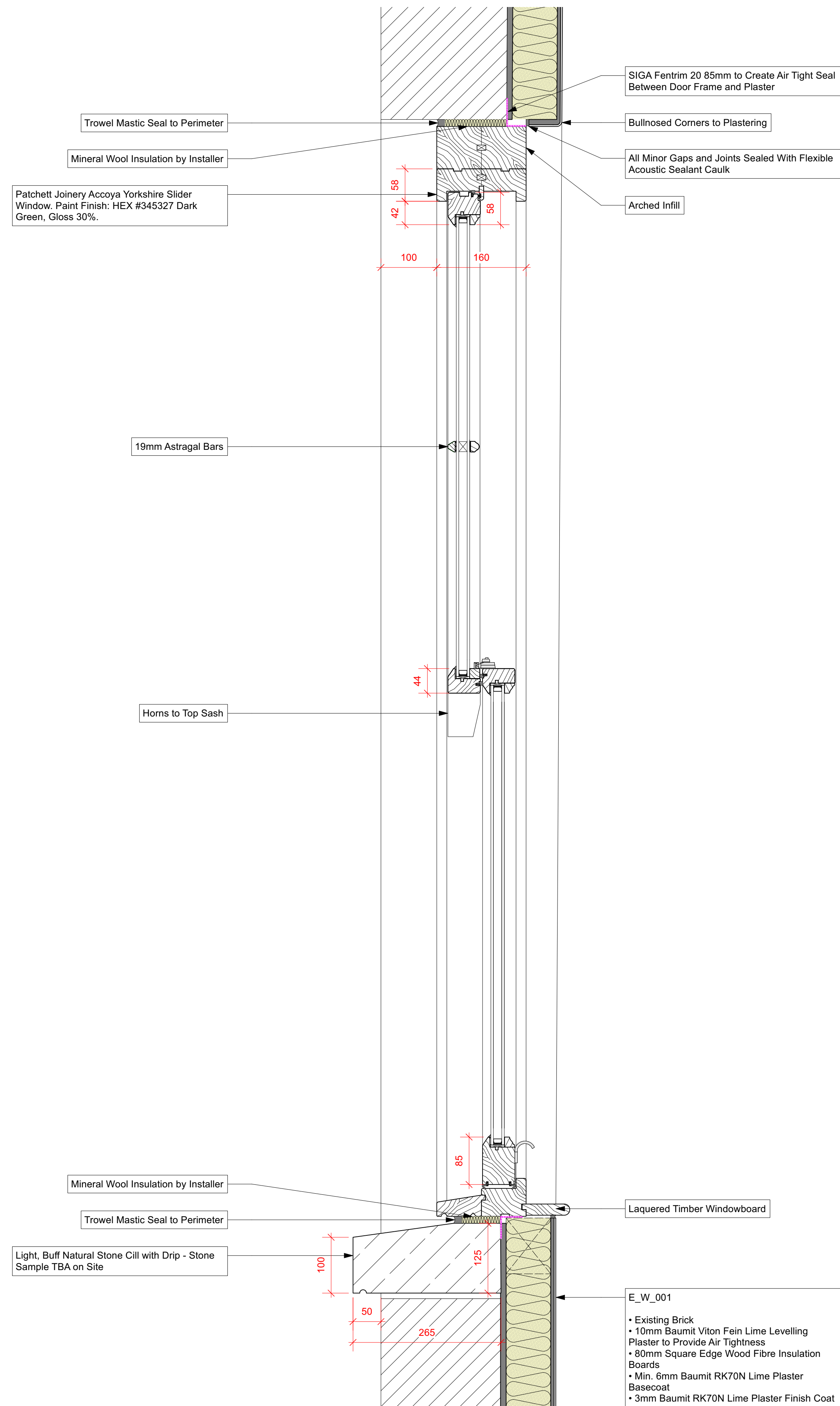
1 Sash Window - Typical Head and Cill Details Scale: 1:5
