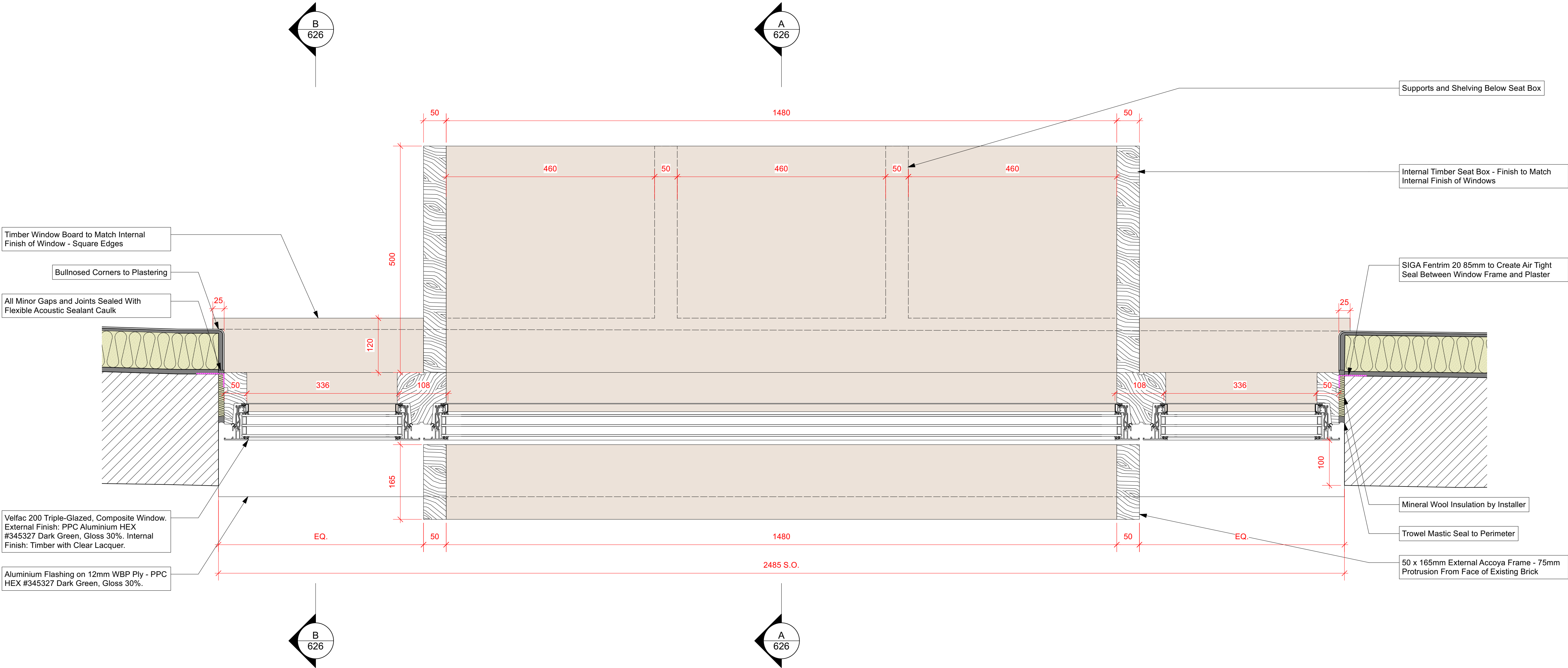
1 W.6 - Plan Detail Scale: 1:5
