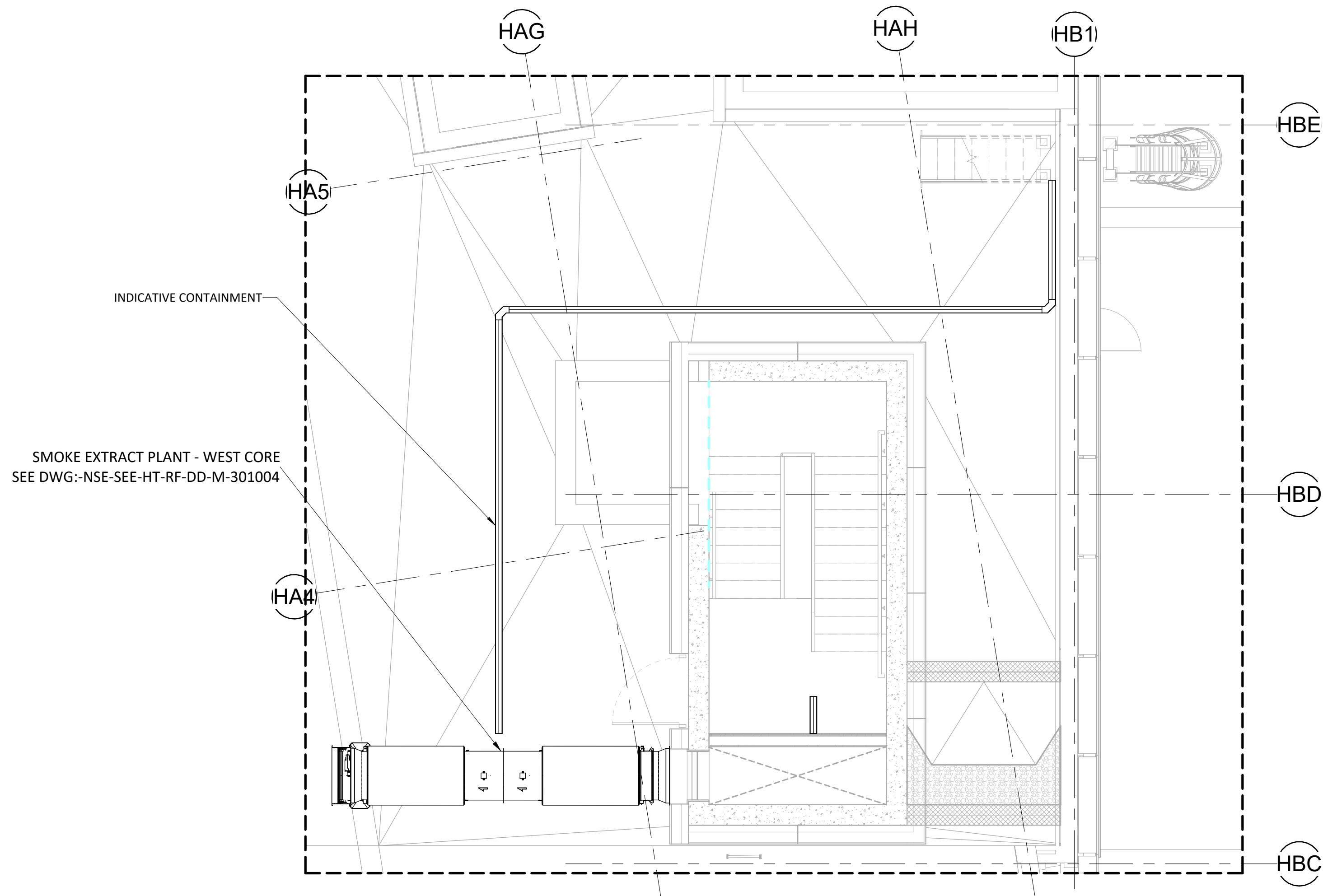
1 WEST CORE 1 : 50
