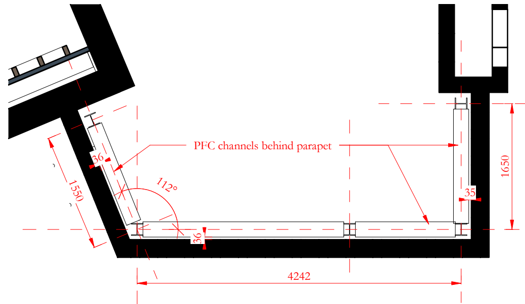
Plan at parapet level
