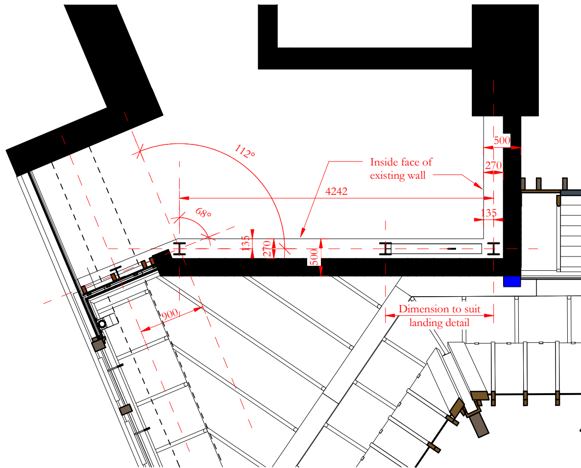
Plan at spreader beam level
