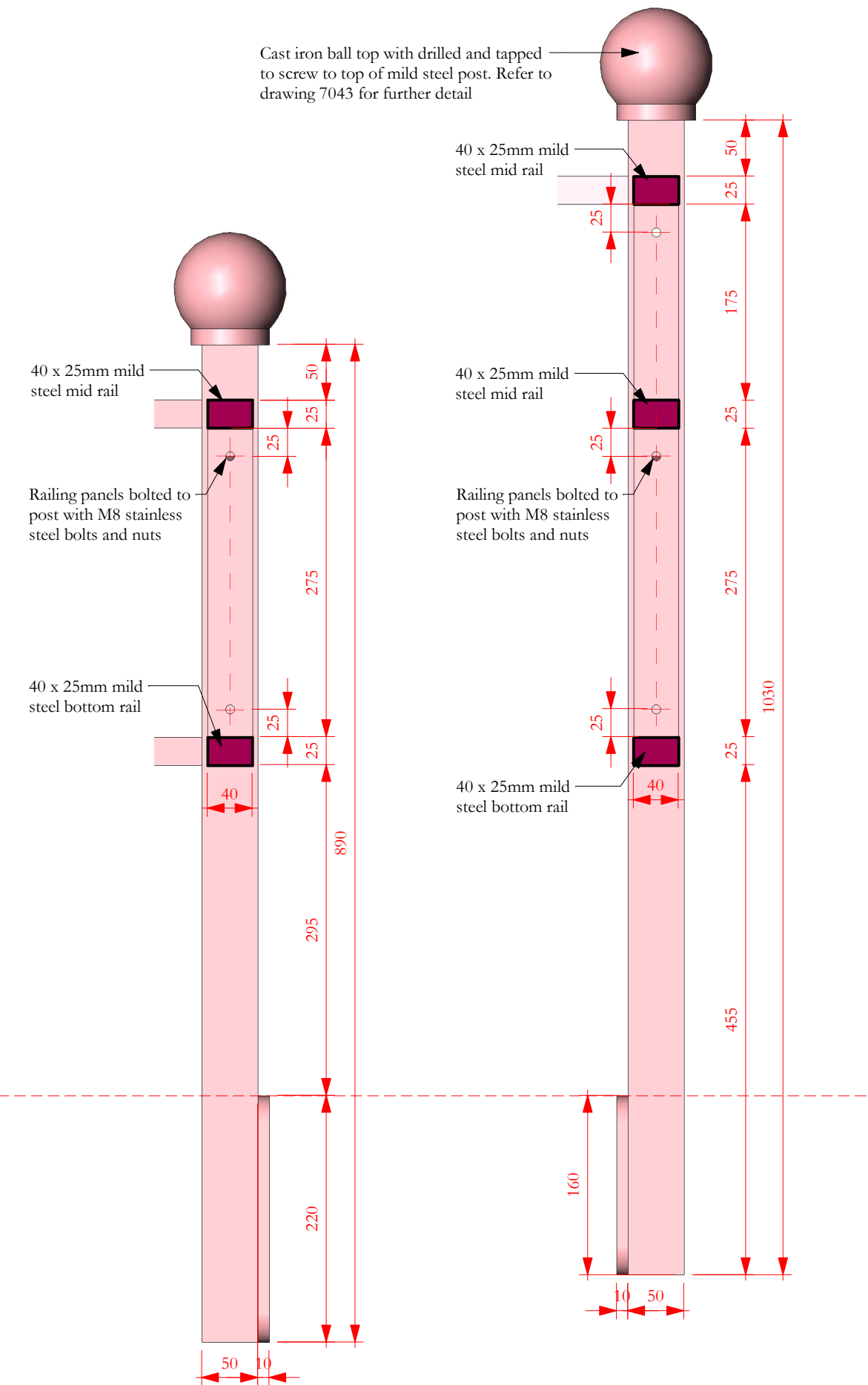
5 - GUARD RAIL POST TYPE 1
