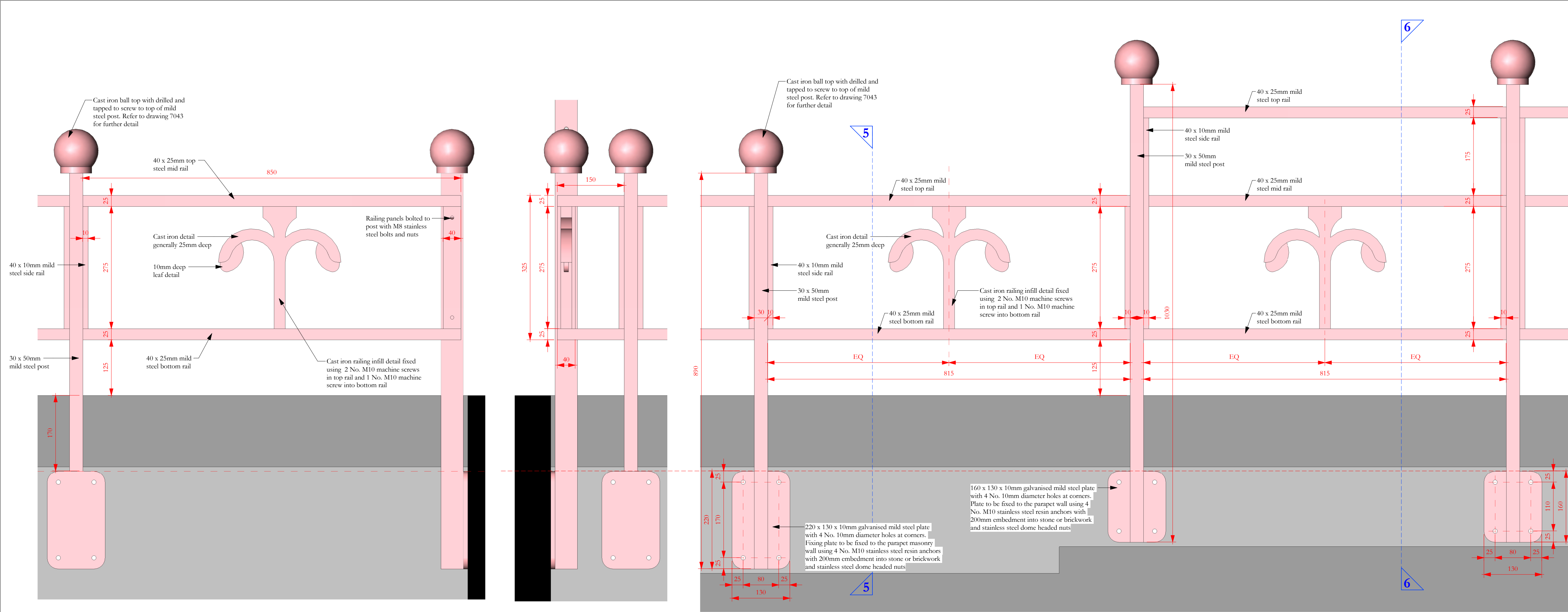
1 - CORNER PANEL LONG ELEVATION
