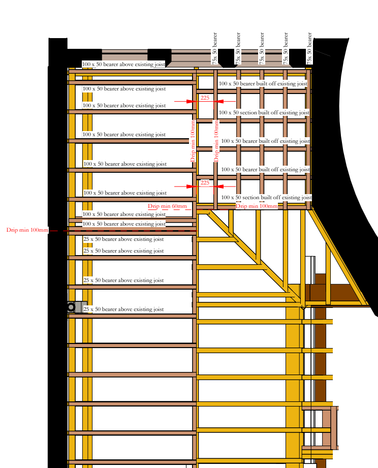
Plan showing proposed structure
