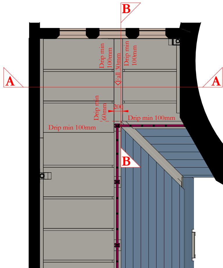
Plan showing proposed roof coverings
