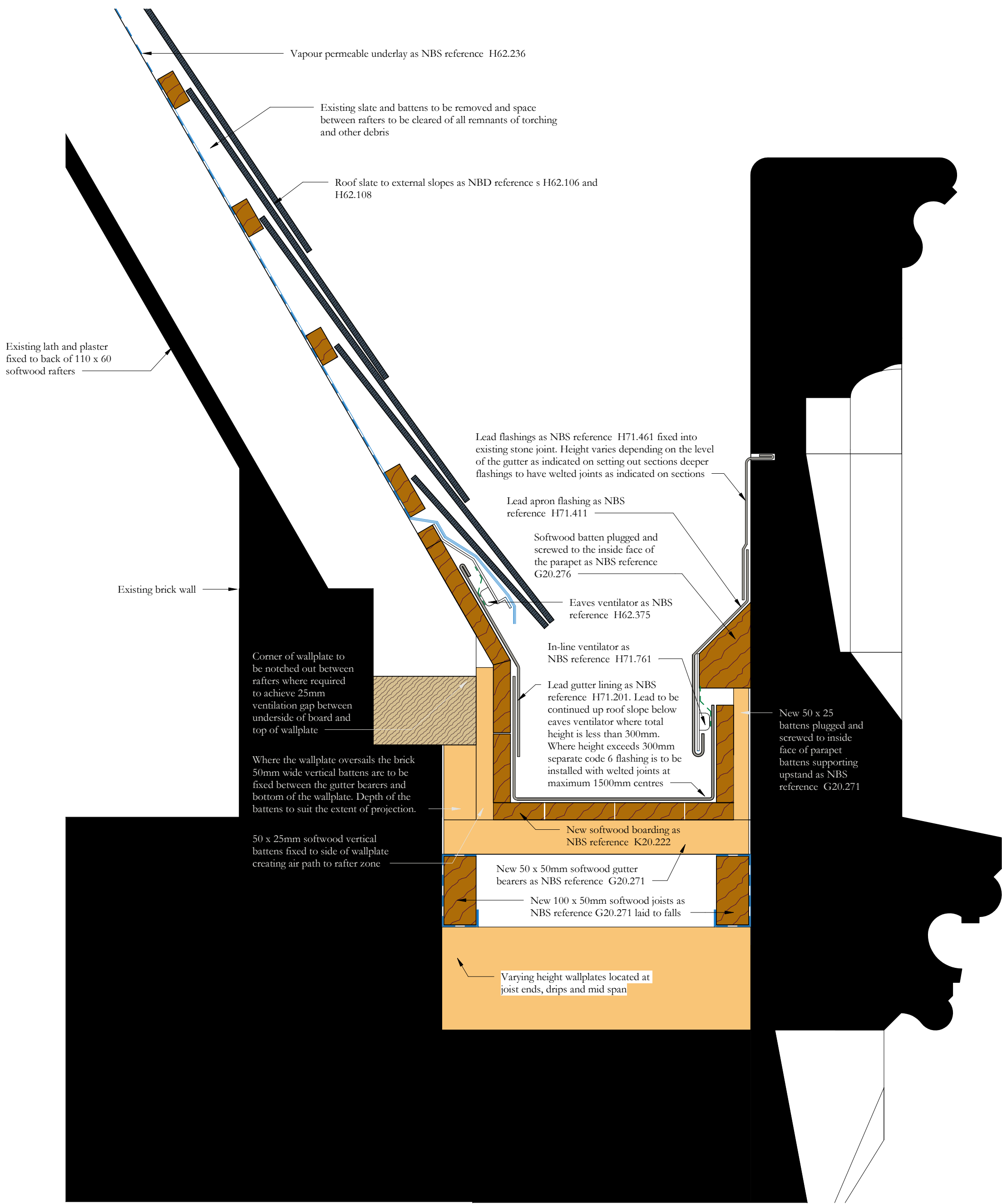
Parapet gutter detail Roofs NR01, NR03, NR05, SR10, SR12, SR13, ER04, ER06, ER08, ER09, WR19, WR20, WR22 and WR27 Scale 1:5
