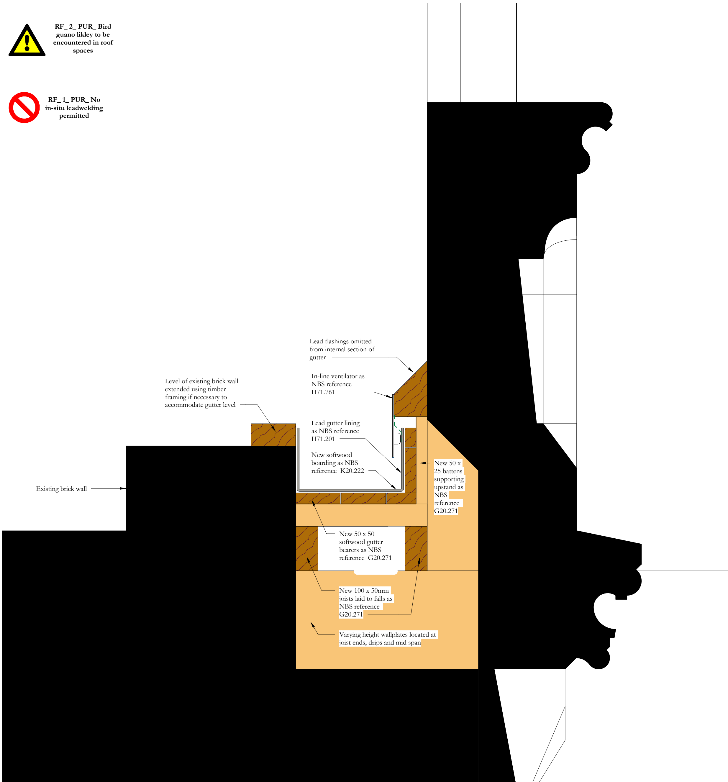
Gutter detail through dormers Roofs NR01, NR03, NR05, SR10, SR12, SR13, ER04, ER06, ER08 and ER09 Scale 1:5
