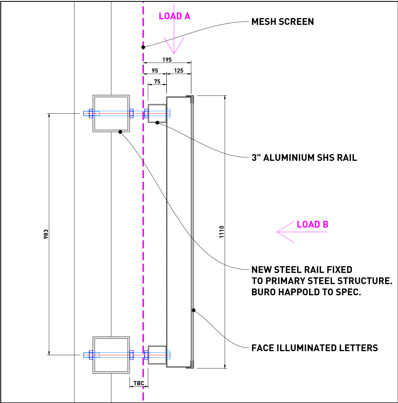
SECTION THROUGH A
