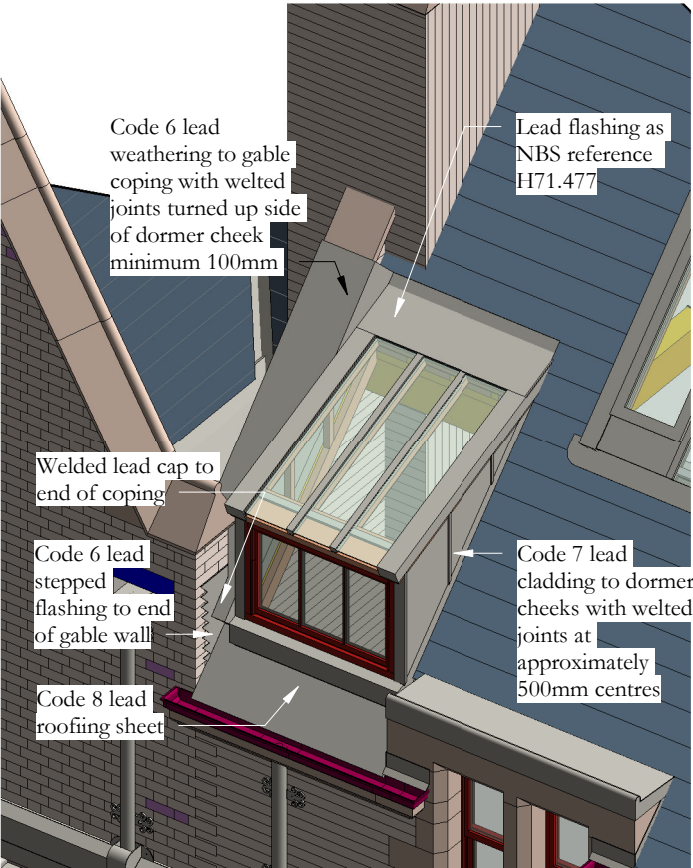
Isometric view of rooflight with roof coverings
