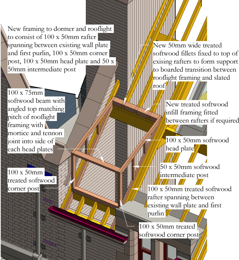
Isometric view of timber framing to dormer
