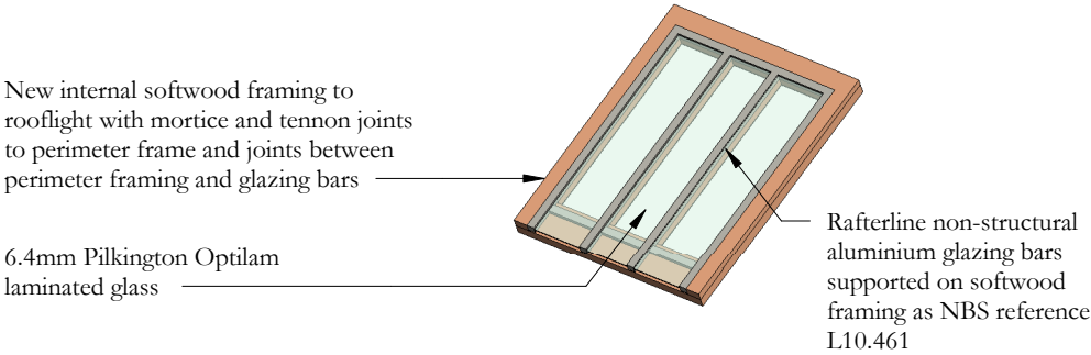
Isometric view of rooflight
