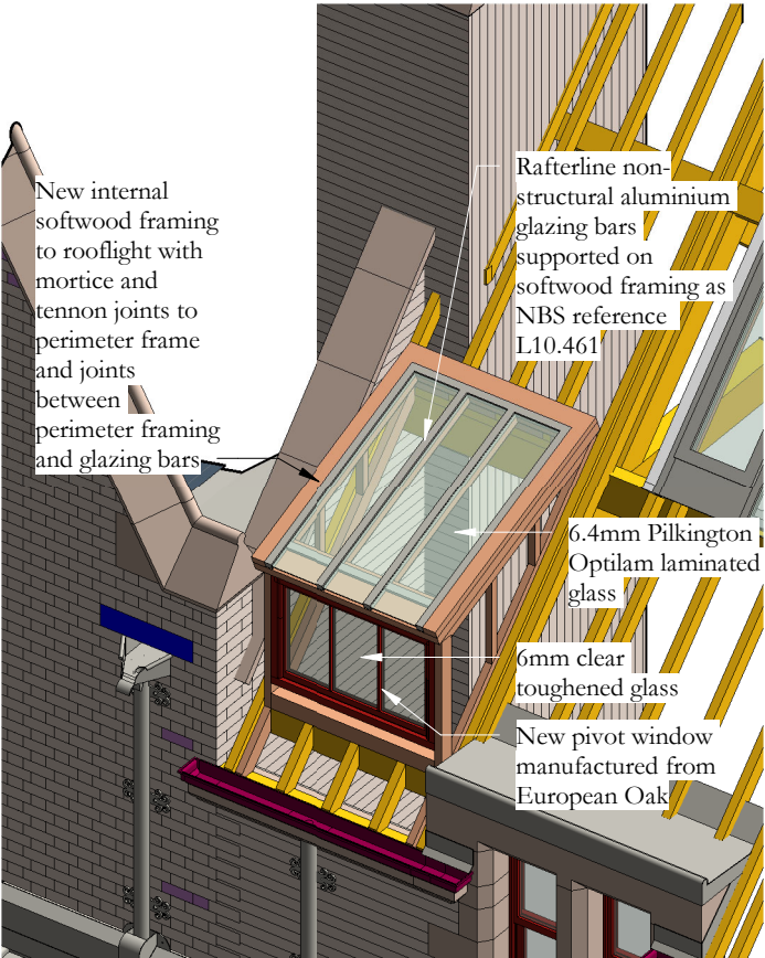
Isometric view of rooflight without roof coverings
