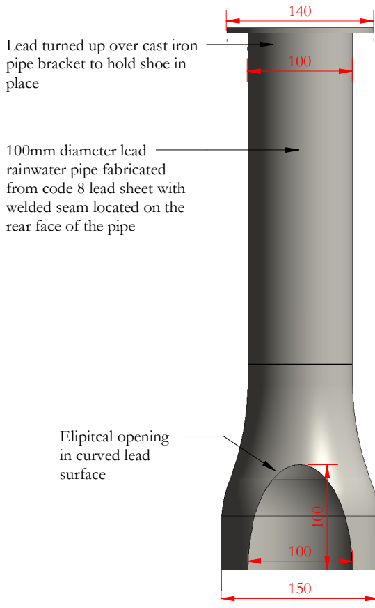
PIPE SHOE SECTION BB
