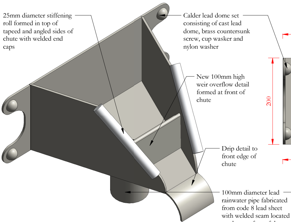
LEAD CHUTE/CATCH PIT AND RAINWATER PIPE ASSEMBLY
