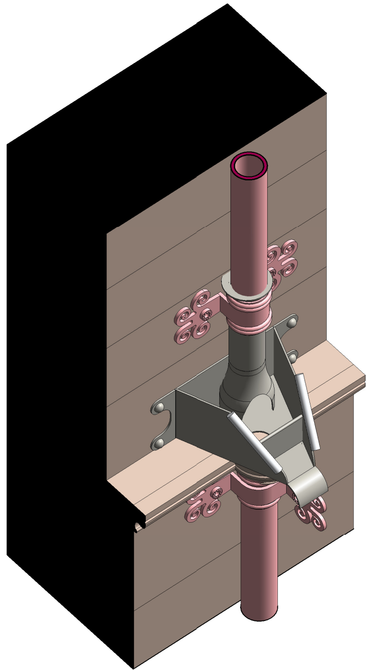
CHUTE ON STRIGHT SECTION OF WALL IN CONTEXT
