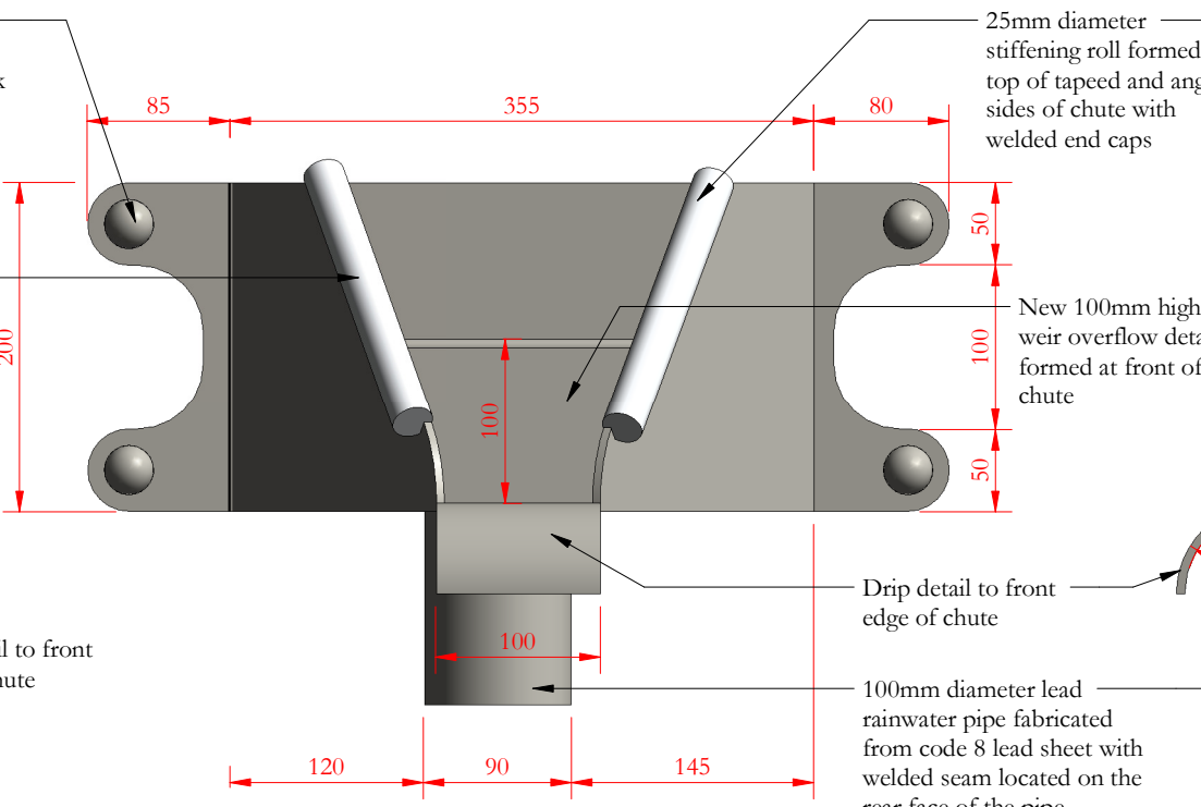
CHUTE/CATCH PIT FRONT ELEVATION
