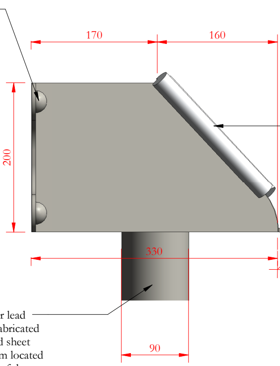
CHUTE/CATCH PIT LEFT SIDE ELEVATION
