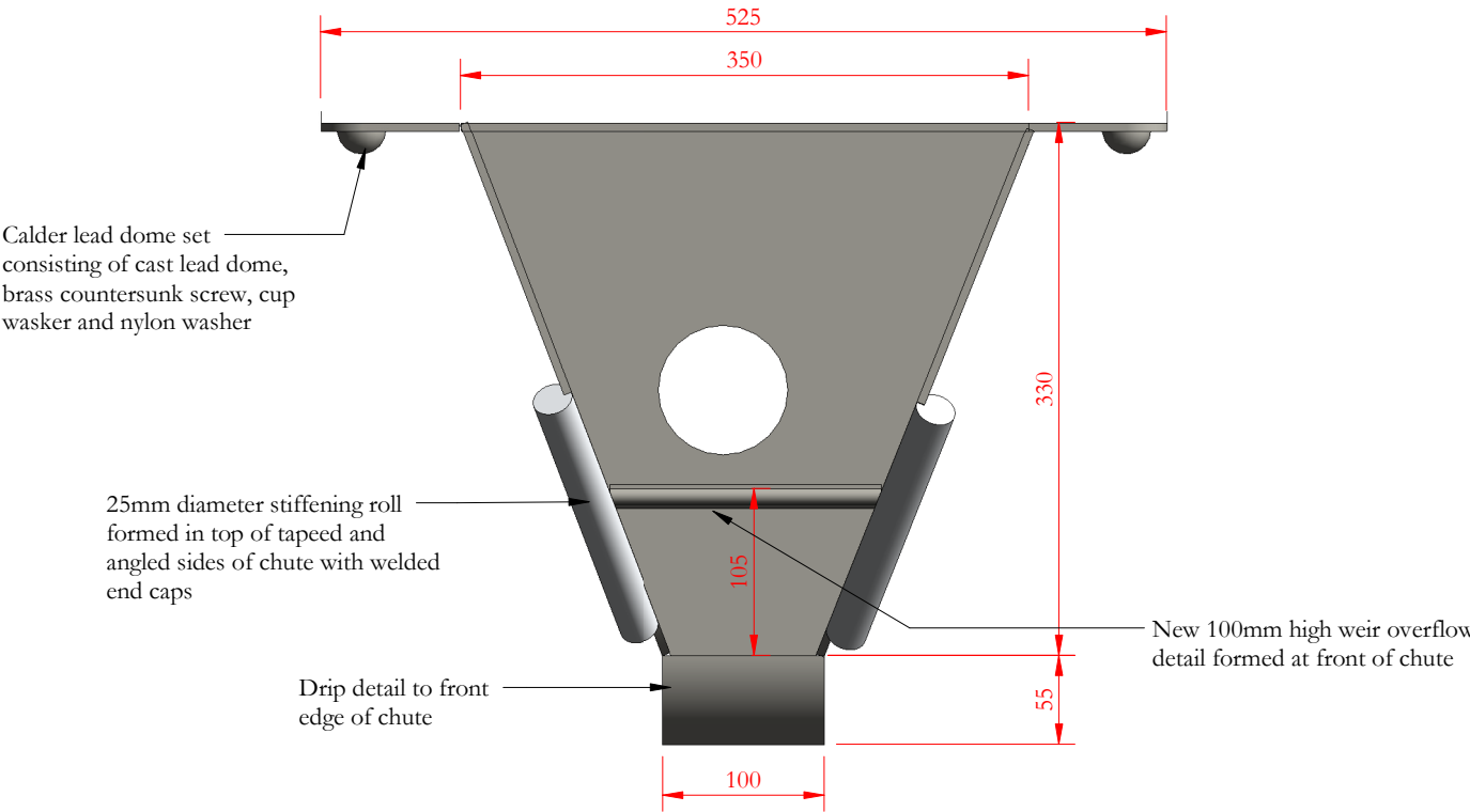
CHUTE/CATCH PIT PLAN
