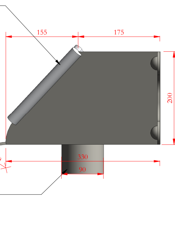
CHUTE/CATCH PIT RIGHT SIDE ELEVATION
