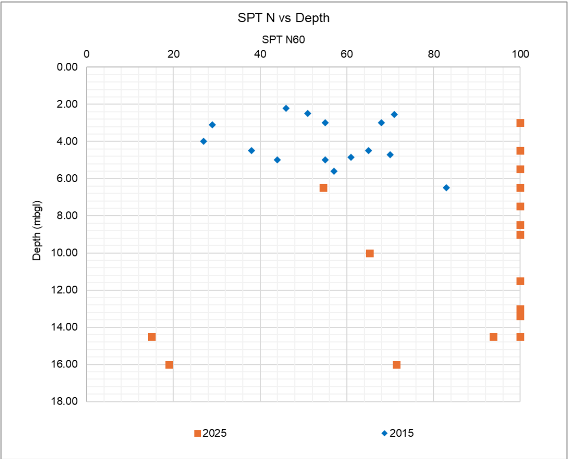
Figure 4-7: SPT N values within Sandstone from 2015 and 2025 investigations
