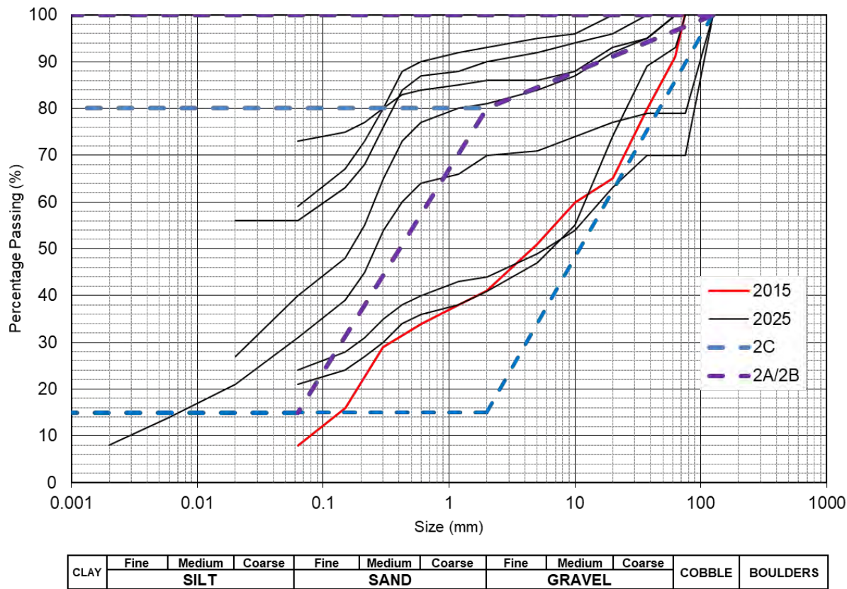
Figure 4-3: Grading Curves for Material Classification - Made Ground, showing bounds of Class 2 materials.
