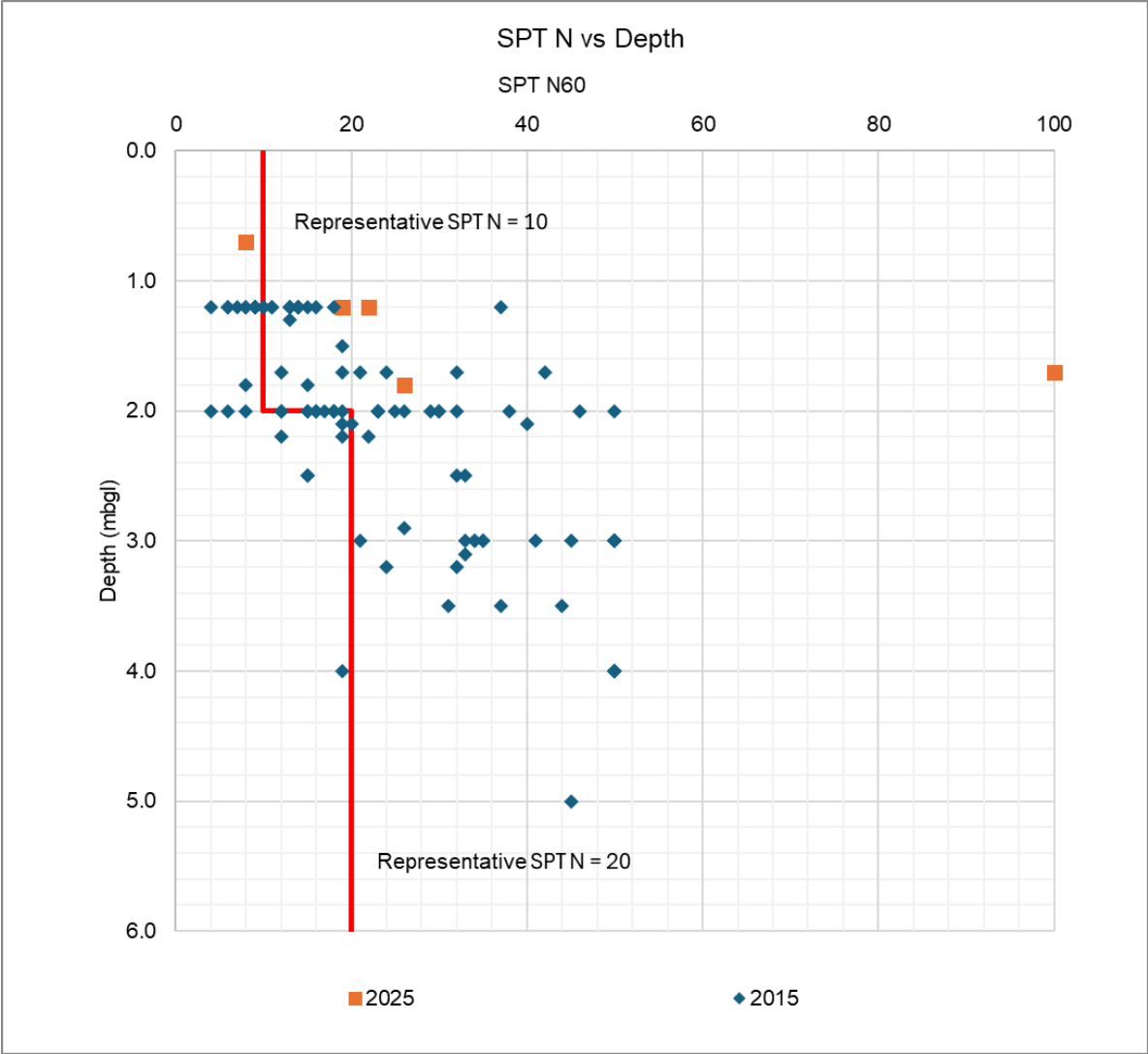
Figure 4-4: SPT N values within Glacial Till from 2015 and 2025 investigations.
