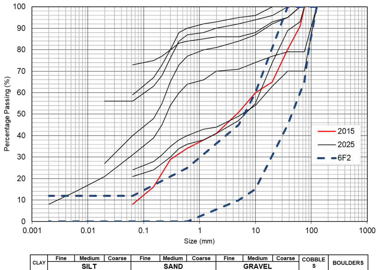
Figure 4-4: Grading Curves for Material Classification - Made Ground, showing bounds of Class 6F2 material.
