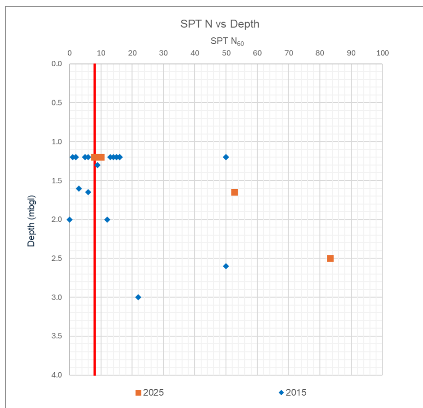
Figure 4-1: SPT N values of 2015 and 2025 investigations within Made Ground.
