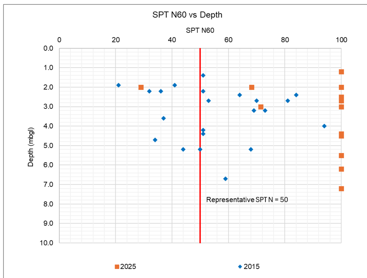
Figure 4-6: SPT N values from 2015 and 2025 investigations within Weathered Sandstone
