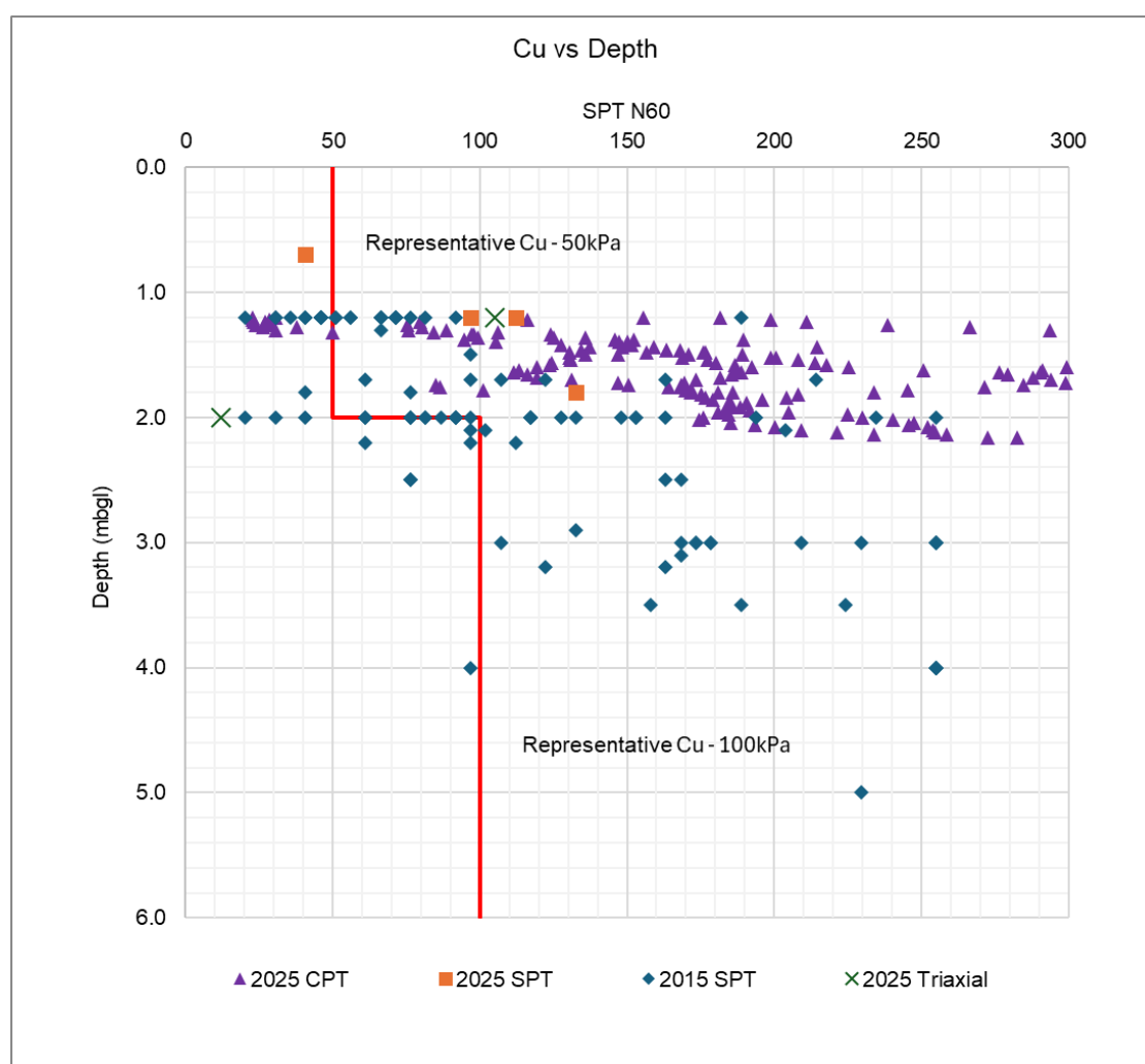
Figure 4-5: c_u derived for Glacial Till from SPT N, CPT, and Triaxial test data
