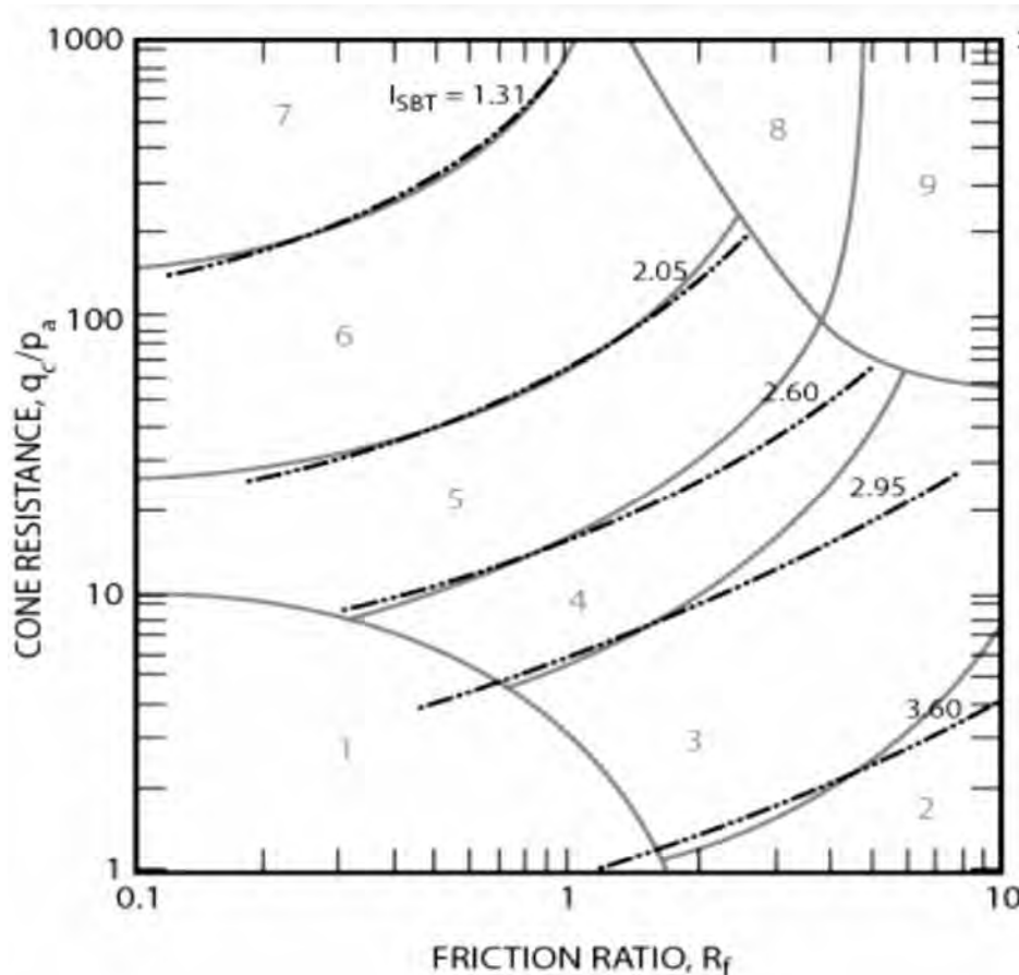
Figure 6-2 Non-normalised SBT chart by Robertson et al. (2010) based on dimensionless cone resistance ( q_c/\text{Pa} ) and friction ratio, R_f , showing contours of SBT index I_{\text{SBT}} (denoted I_c on the test plots). The chart is equally applicable to normalised tip resistance ( Q_t , Q_{tn} ) and normalised friction ratio ( F_r ) values using the same dimensionless scales.
