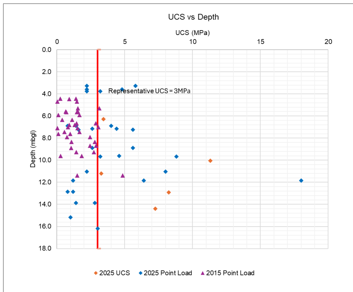
Figure 4-8: UCS results from 2015 and 2025 ground investigation
