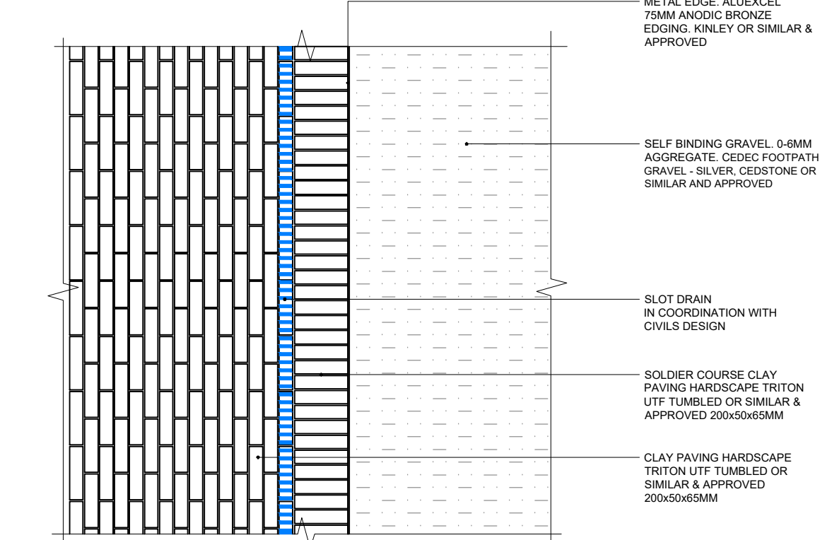
06B 601 METAL EDGE FOR CLAY PAVING AND SELF BINDING GRAVEL PLAN
