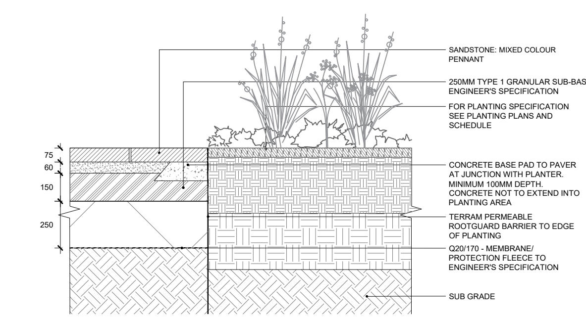
07A 601 EDGE TO PLANTING AGAINST SANDSTONE SECTION
