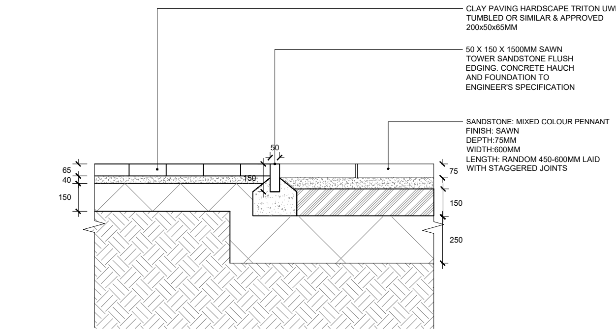
02A 601 ET02 - EDGE TO CLAY PAVING AGAINST SANDSTONE SECTION
