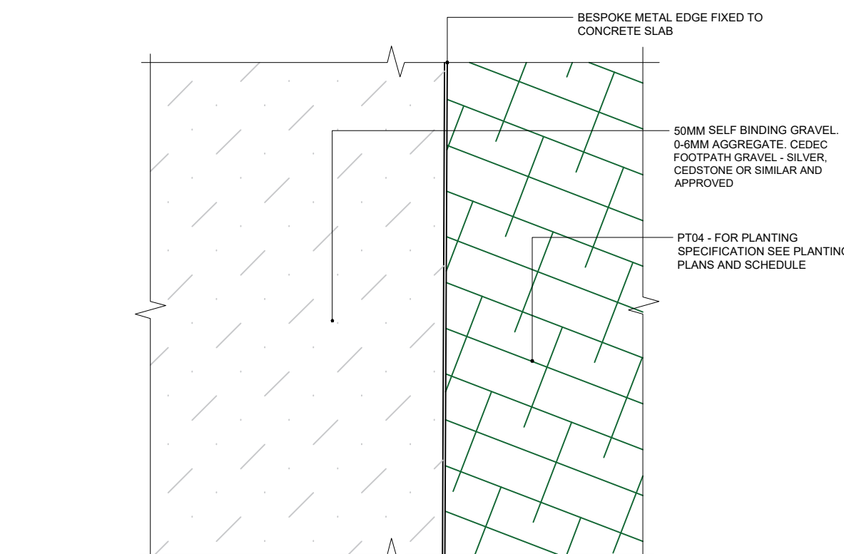
04B 601 ET04 - METAL EDGE FOR SELF BINDING GRAVEL PLAN
