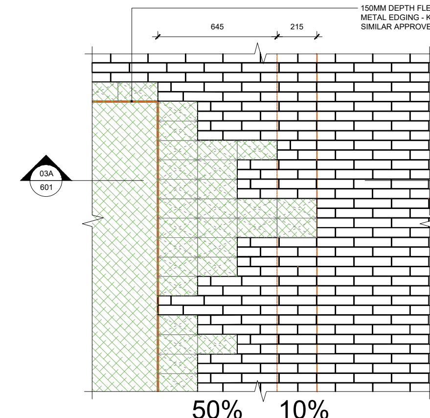
03B 601 ET03 - PLANTING AGAINST GREEN BRICK PLAN
