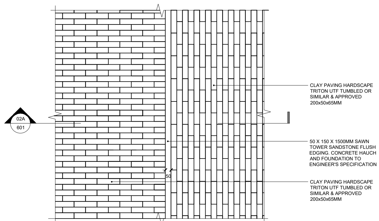
02C 601 ET02 - CLAY PAVING AGAINST CLAY PAVING PLAN
