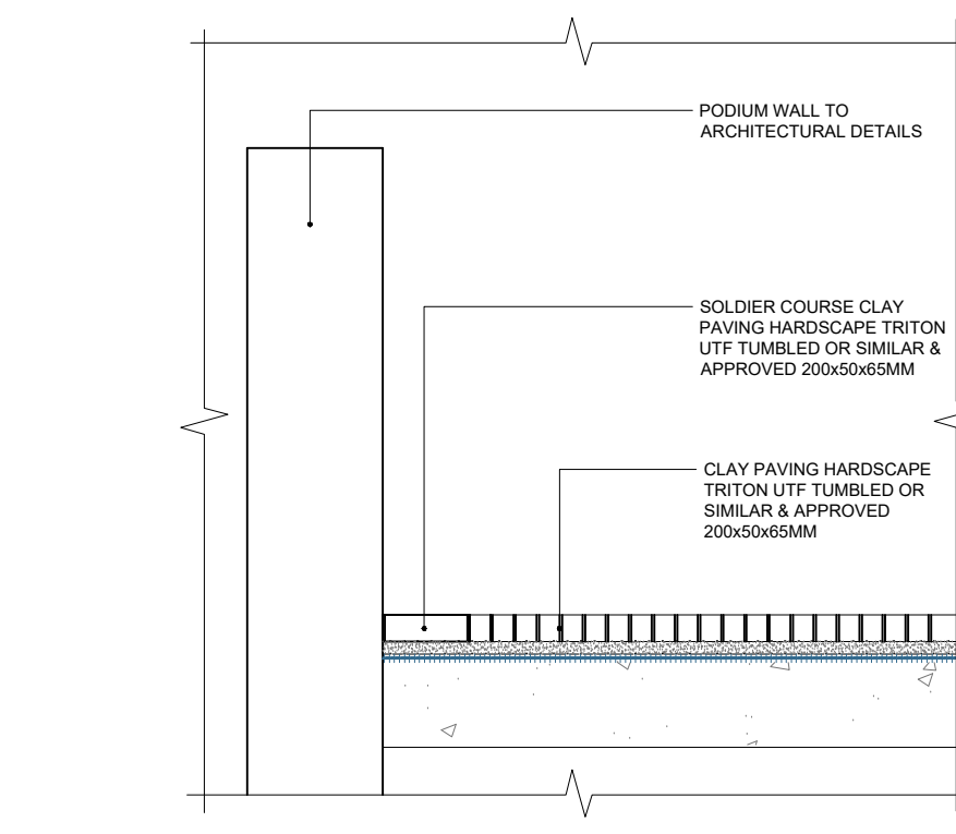
05 601 SOLDIER COURSE CLAY PAVING PODIUM PERIMETER SECTION
