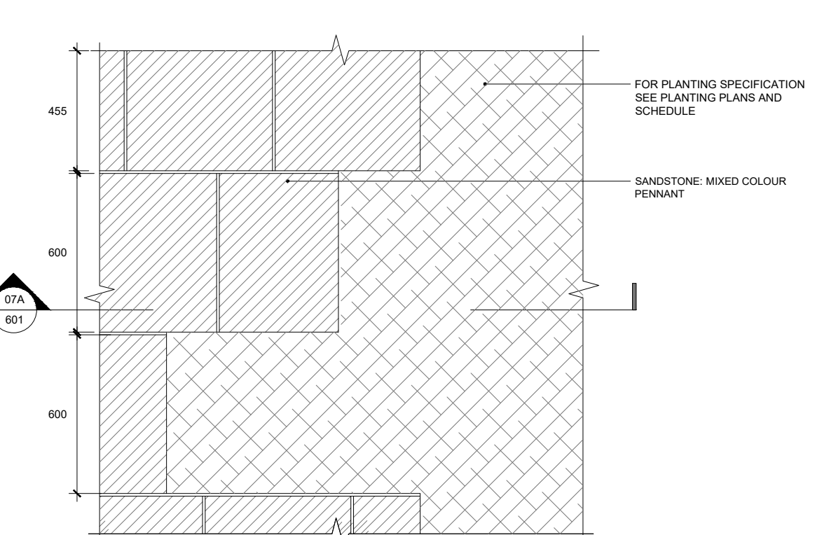
07B 601 EDGE TO PLANTING AGAINST SANDSTONE PLAN
