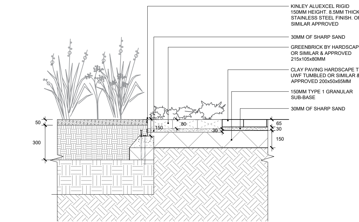
03A 601 ET03 - PLANTING AGAINST GREEN BRICK SECTION
