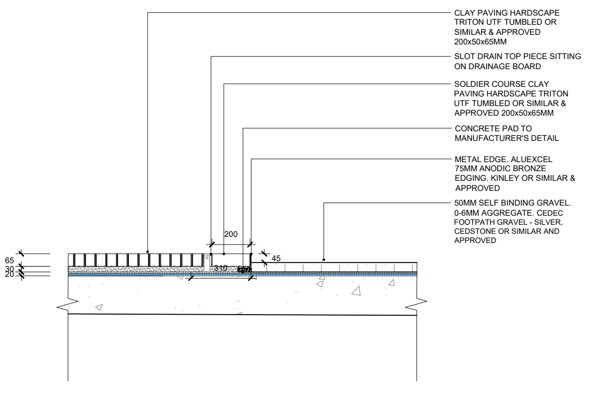
06A 601 METAL EDGE FOR CLAY PAVING AND SELF BINDING GRAVEL SECTION
