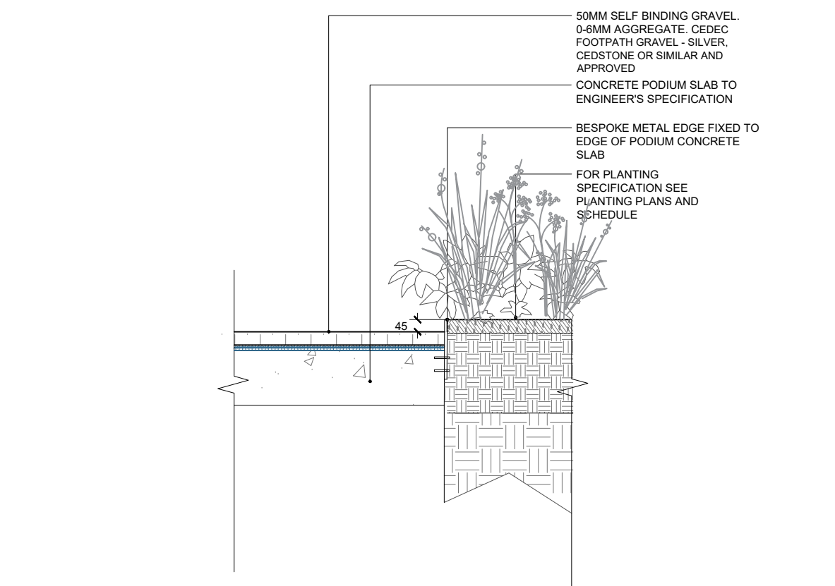
04A 601 ET04 - METAL EDGE FOR SELF BINDING GRAVEL SECTION
