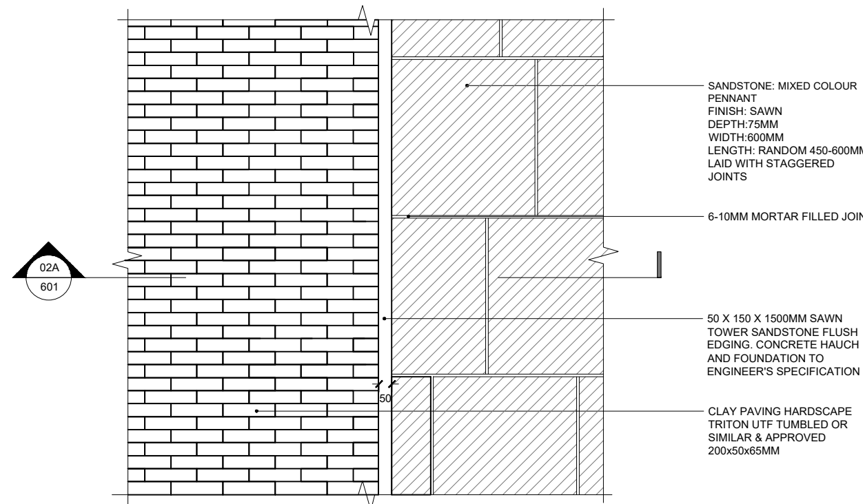
02B 601 ET02 - CLAY PAVING AGAINST SANDSTONE PLAN
