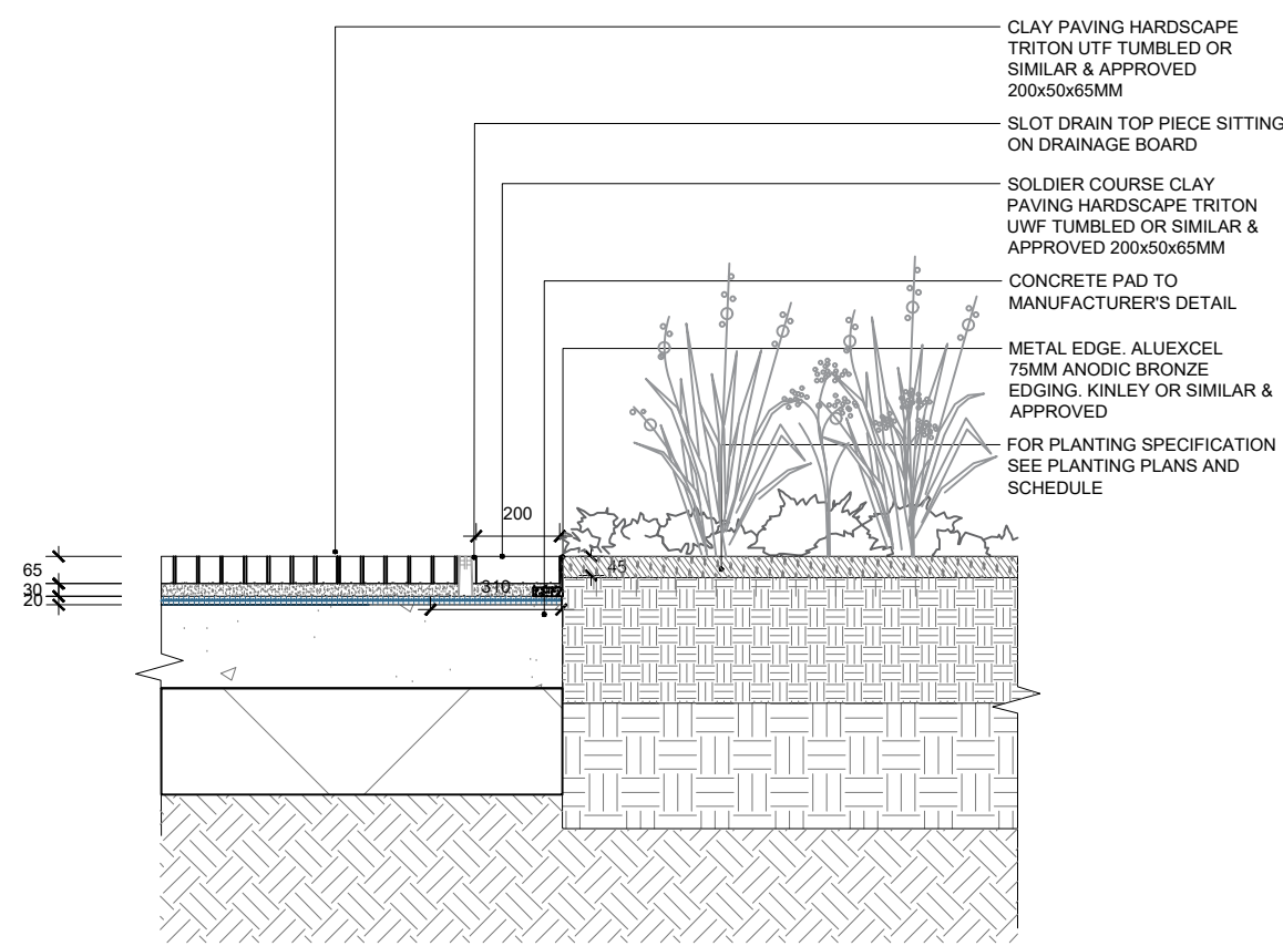
01A 601 ET01 - METAL EDGE FOR CLAY PAVING AND PLANTING SECTION
