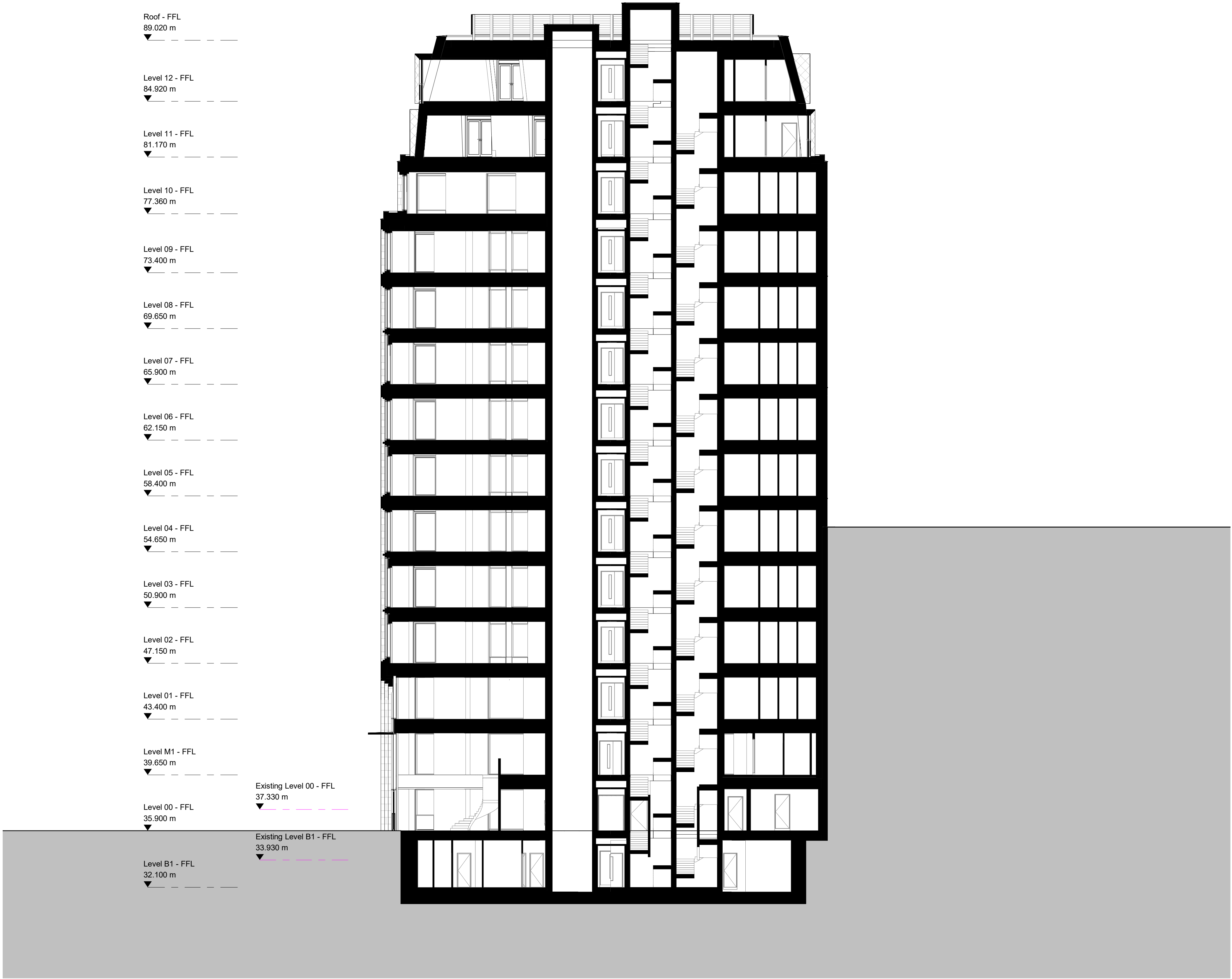
01 Proposed Section BB 1 : 150
