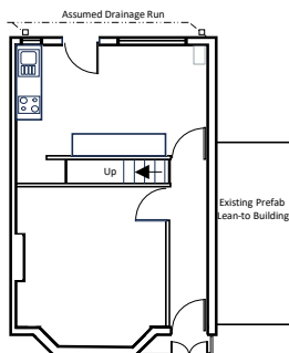
Existing GF Plan 1: 100
