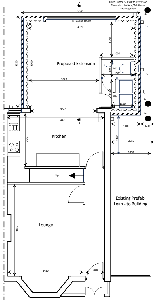
Proposed GF Plan 1: 50
