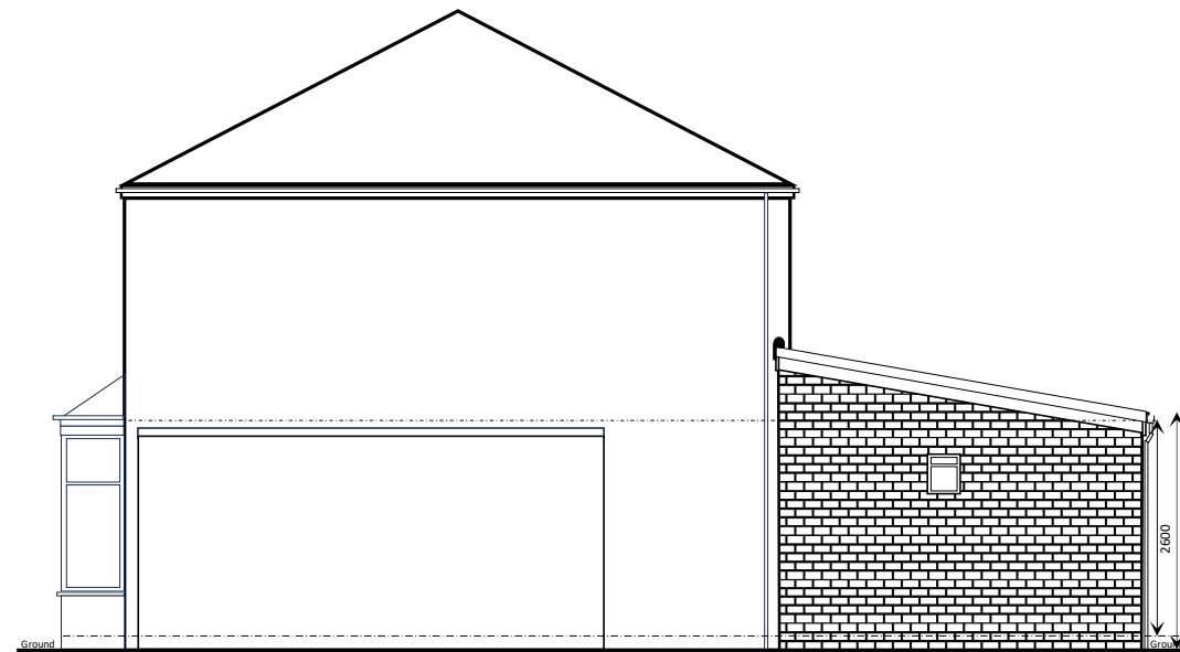
Proposed Side Elevation 1: 50
