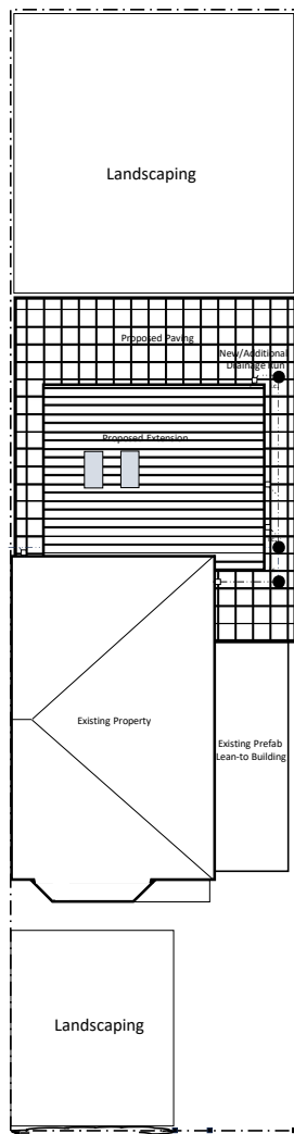
Proposed Site Plan 1: 100
