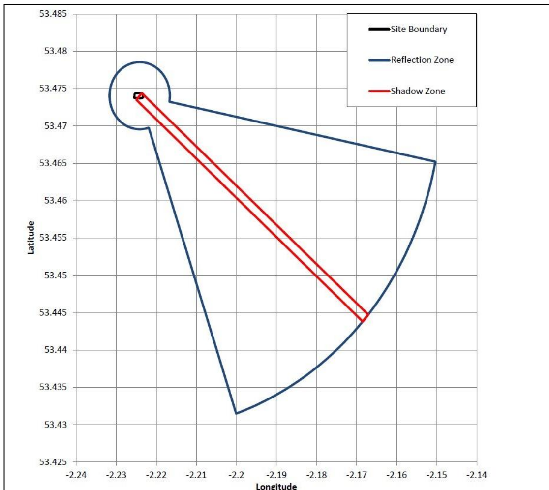
Figure 4 Interference areas
