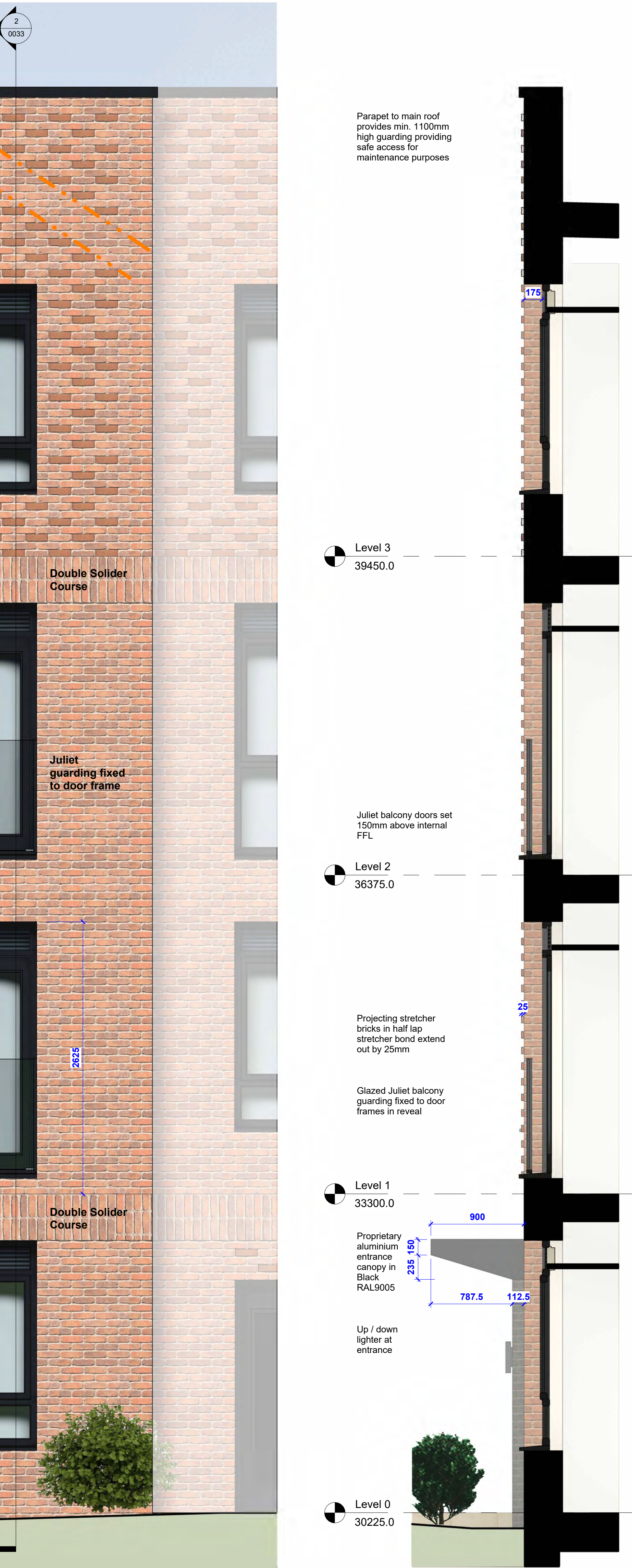
2 Bay Study Section 1 : 25
