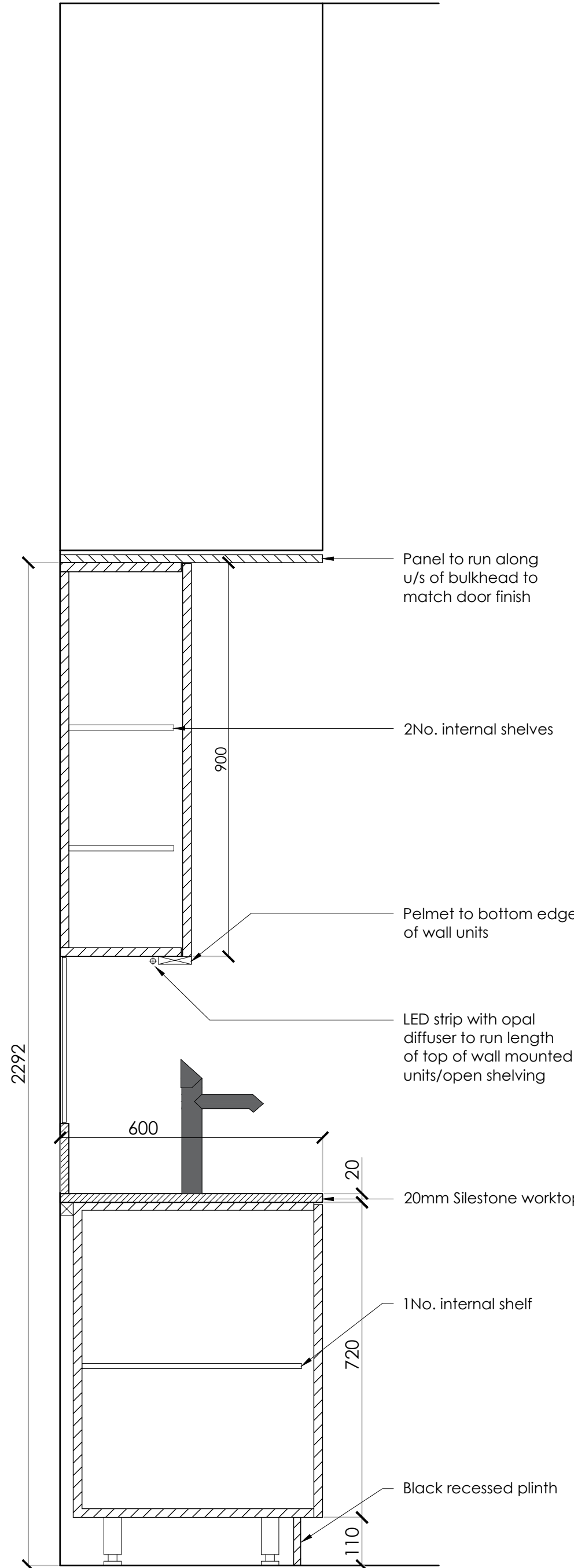
SECTION F-F SCALE 1:10
