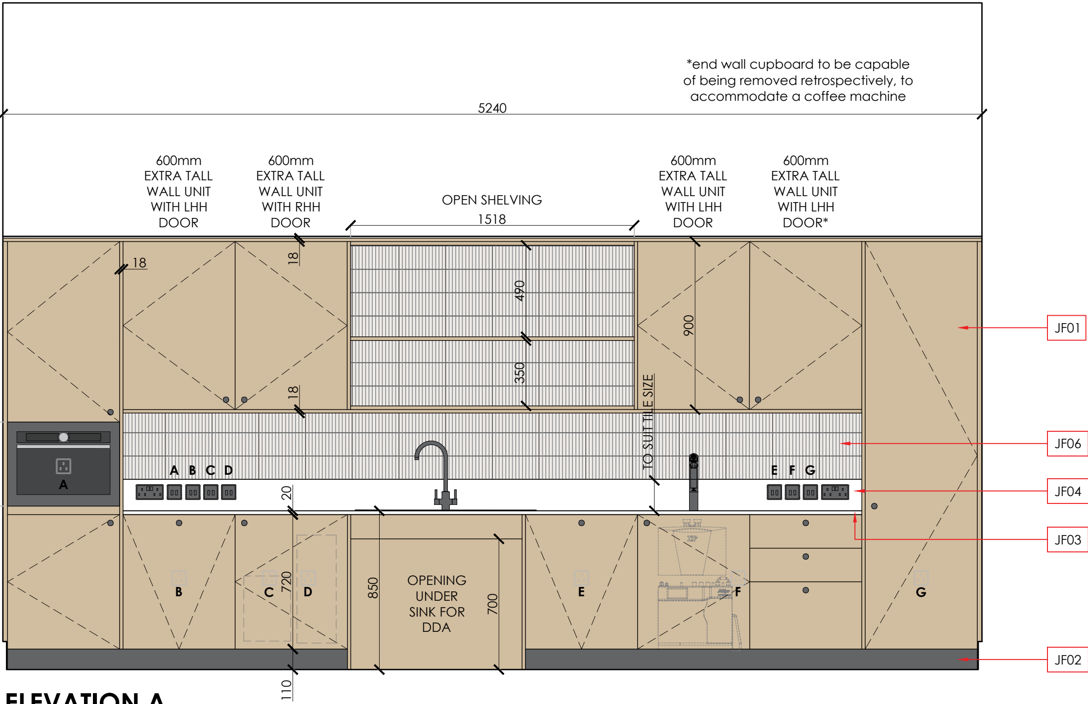
ELEVATION A TEAPOINT
