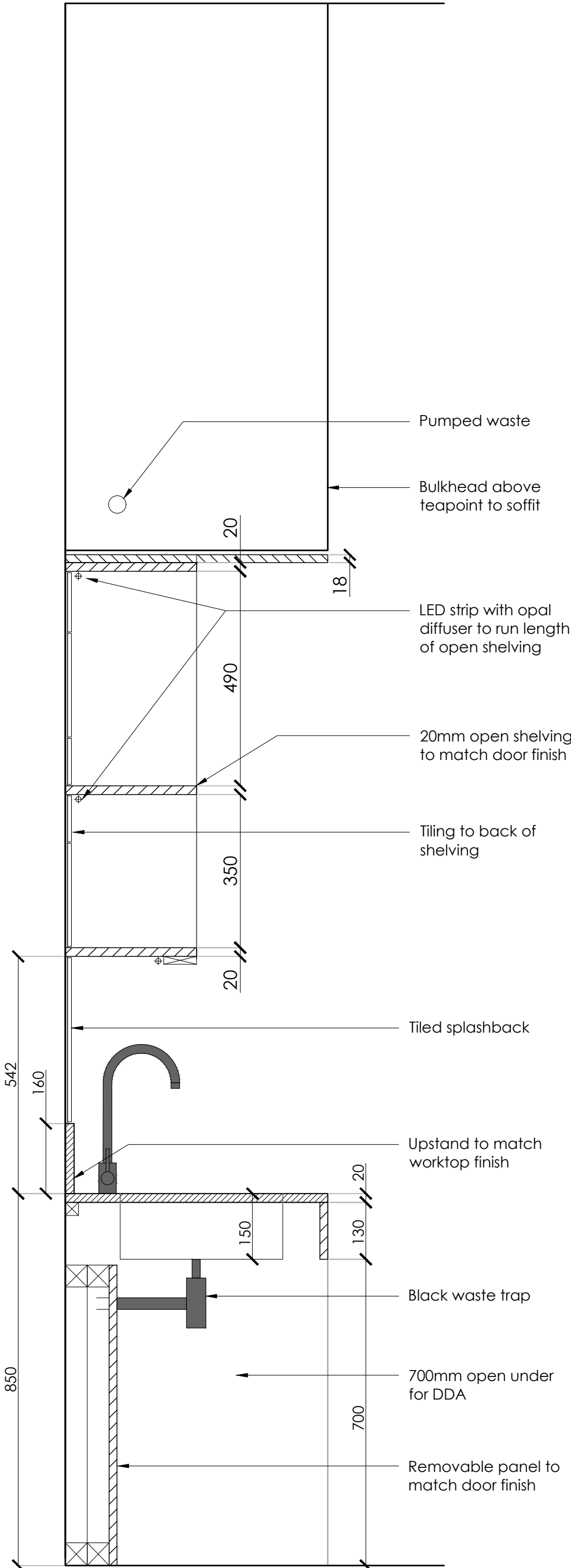
SECTION E-E SCALE 1:10
