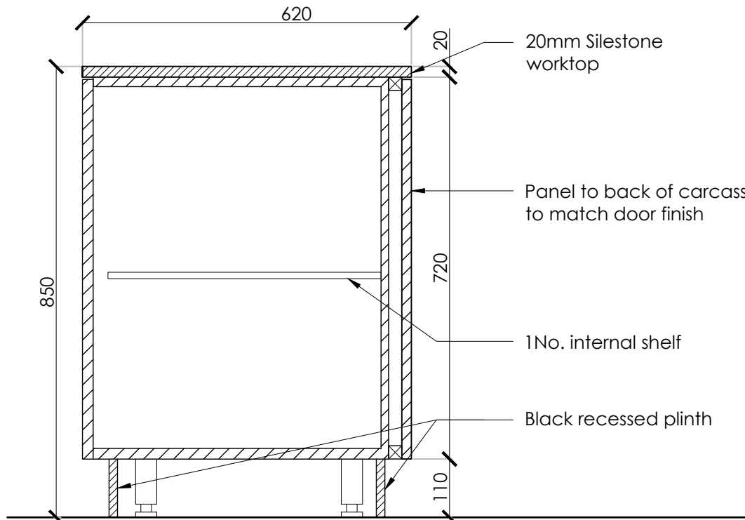
SECTION G-G SCALE 1:10
