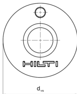
Sealing washer
