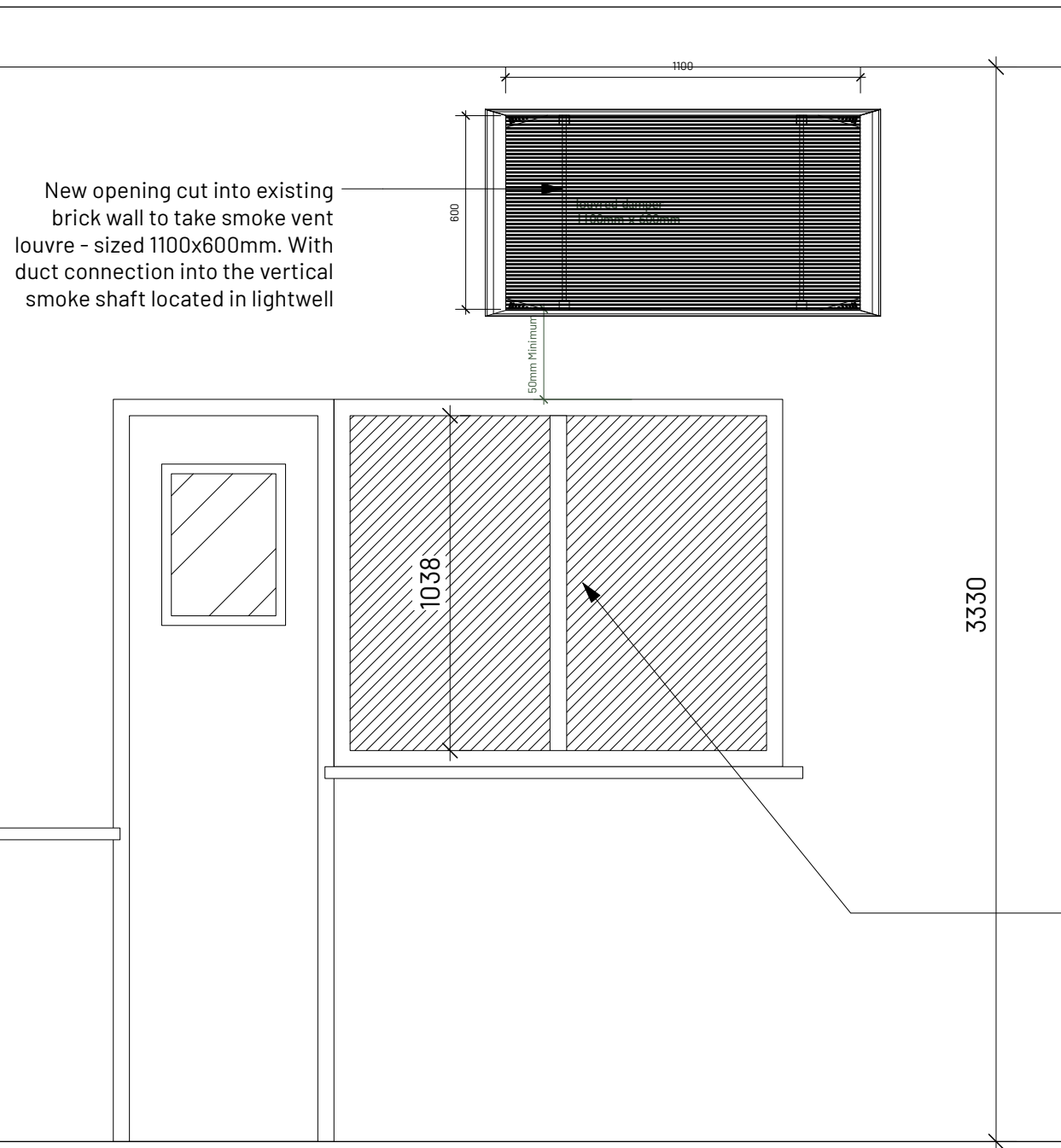
4th Floor Internal Elevation Scale: 1:20
