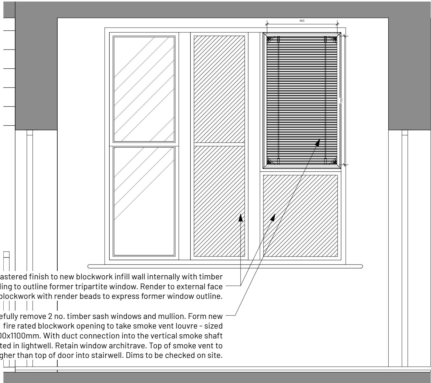
Typical Internal Elevation (Floors 1-3) Scale: 1:20
