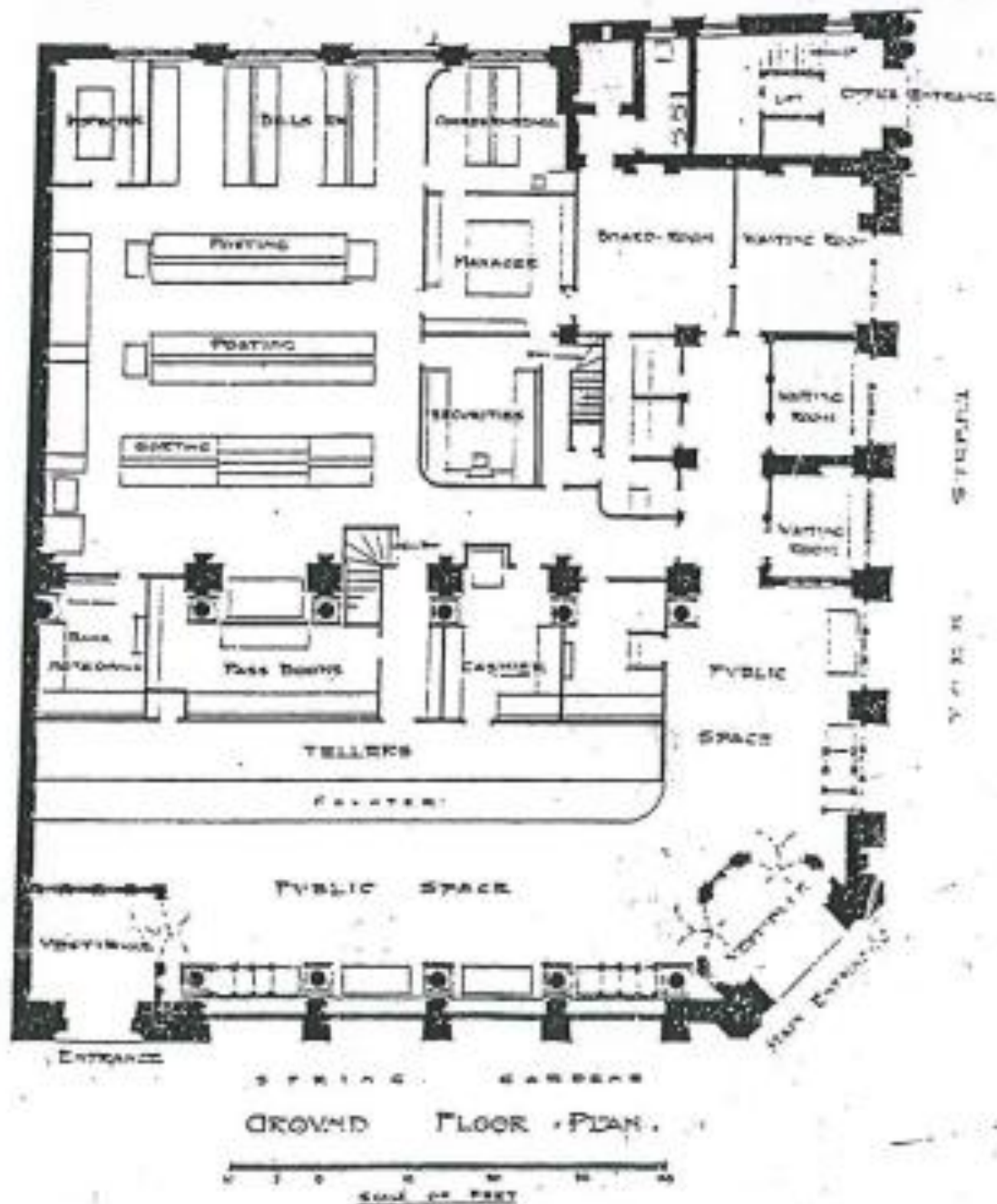
1-3 York Street Manchester Plan of ground floor Banking Hall & Clerks Room The Builders Journal July 10 1907
