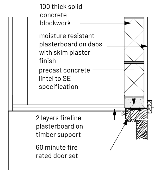
7 LG 1B Door Head Detail Scale: 1:10
