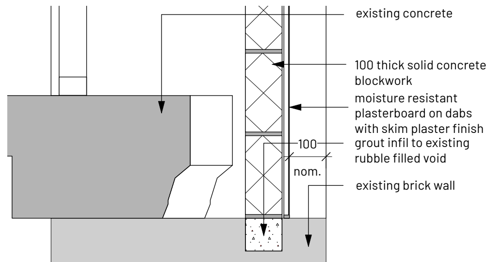
6 LG 1B Partition Base Detail Scale: 1:10
