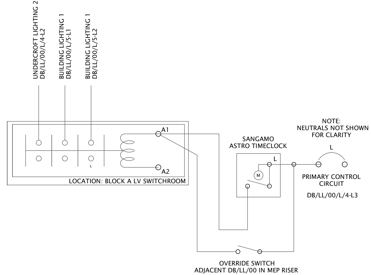
61 - Photocell T/C External Lighting Control Detail (Block B)
