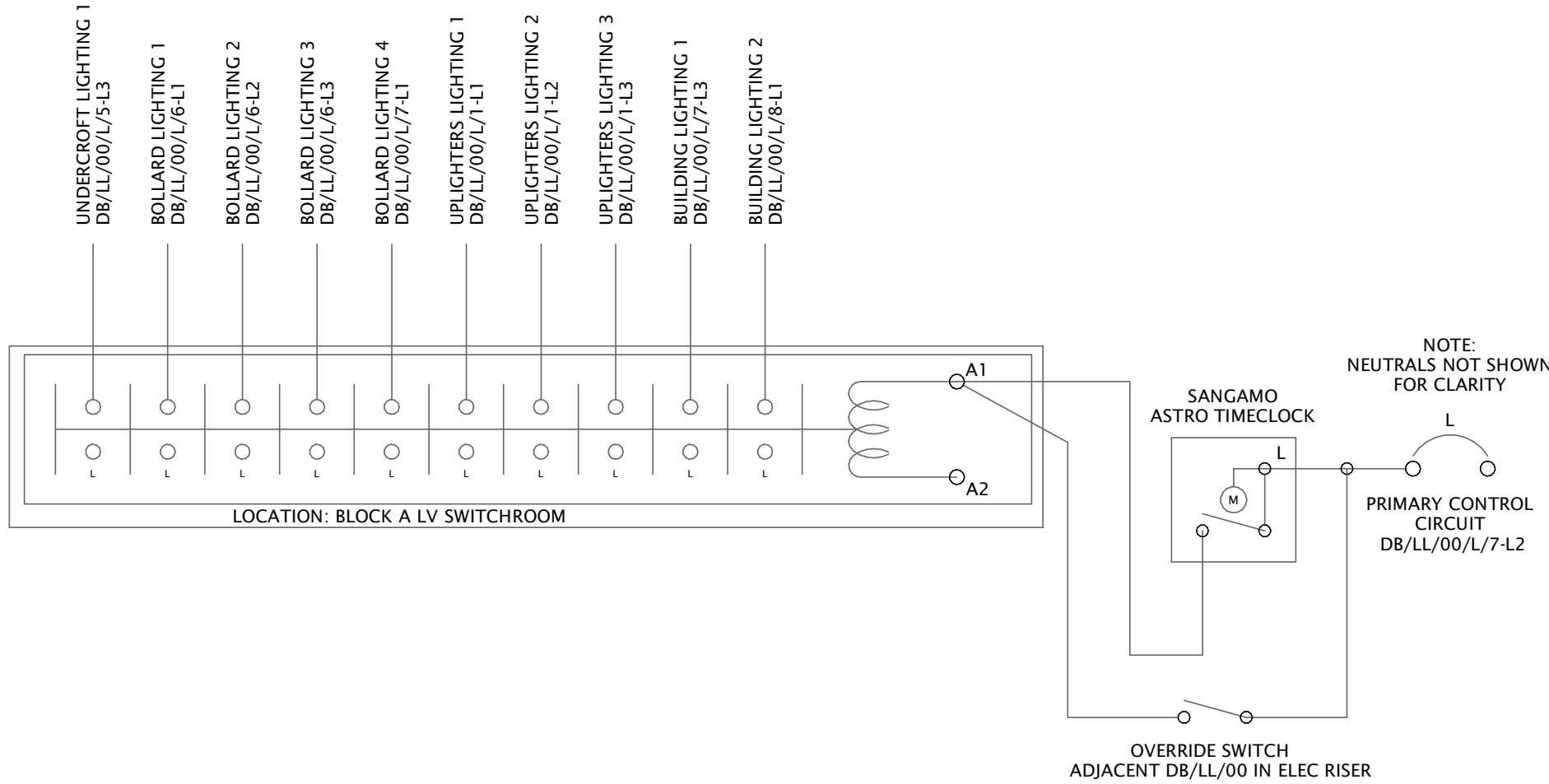
61 - Photocell T/C External Lighting Control Detail (Block A)
