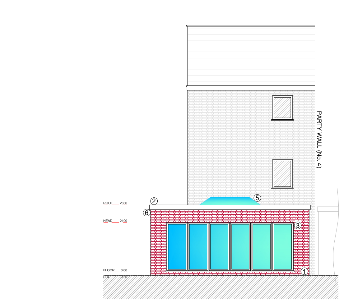
REAR ELEVATION
