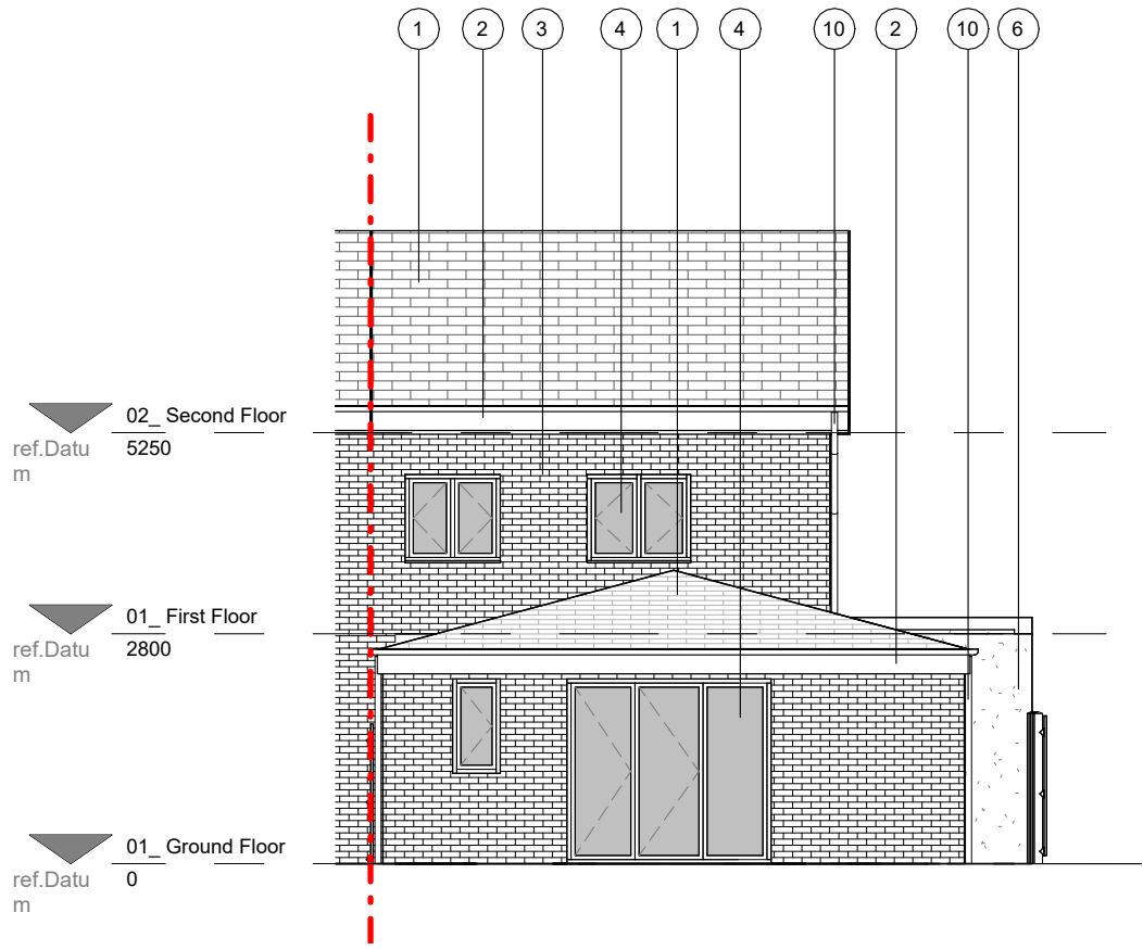
South Elevation 1 : 100
