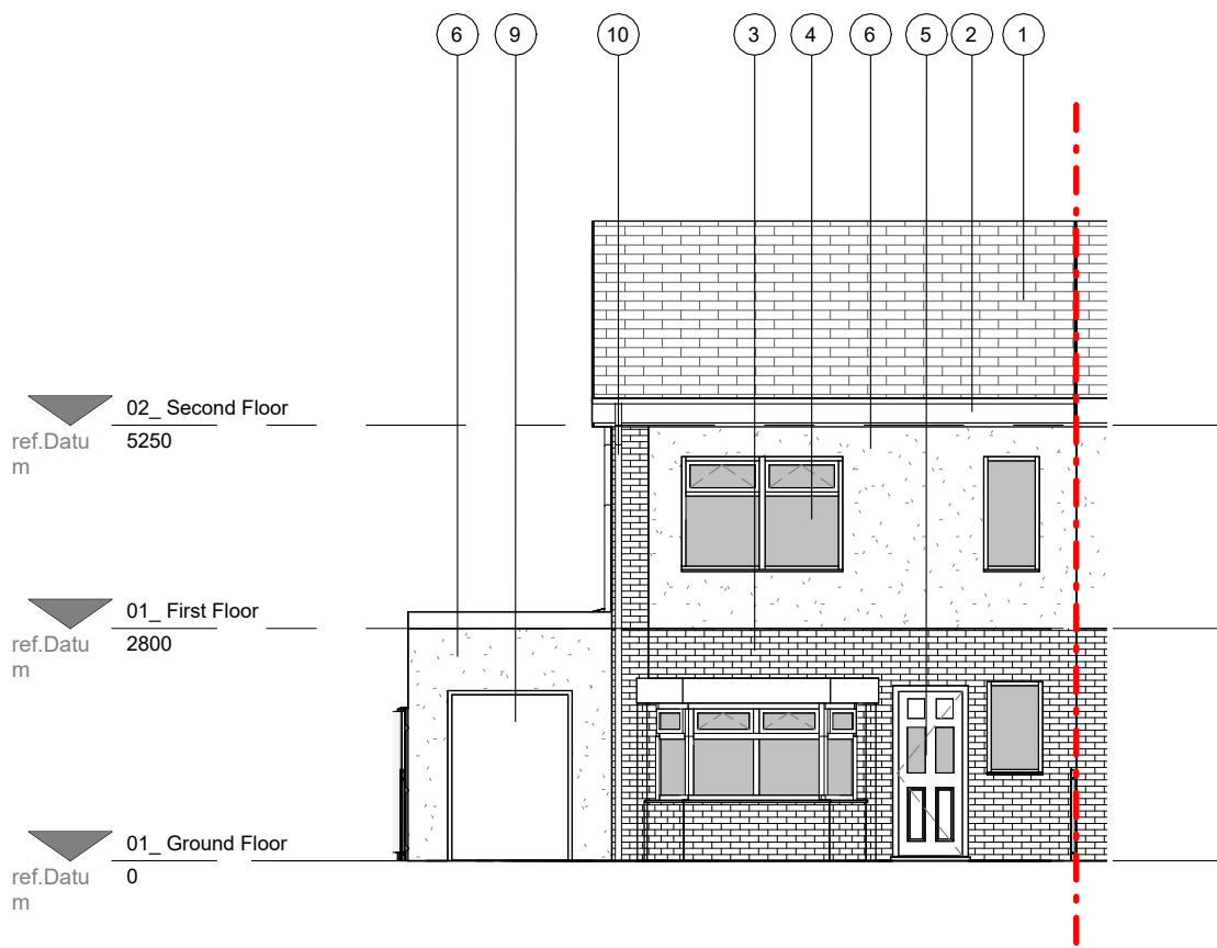
North Elevation 1 : 100
