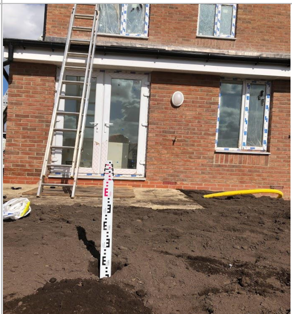
Depth of Cover System in Relation to Plot
