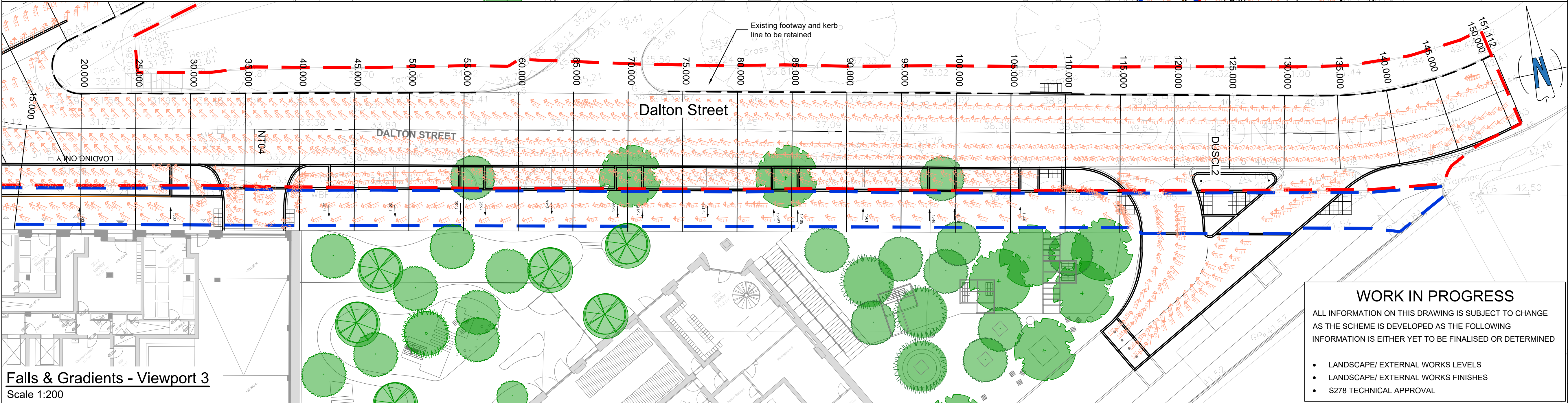
Falls & Gradients - Viewport 2 Scale 1:200
