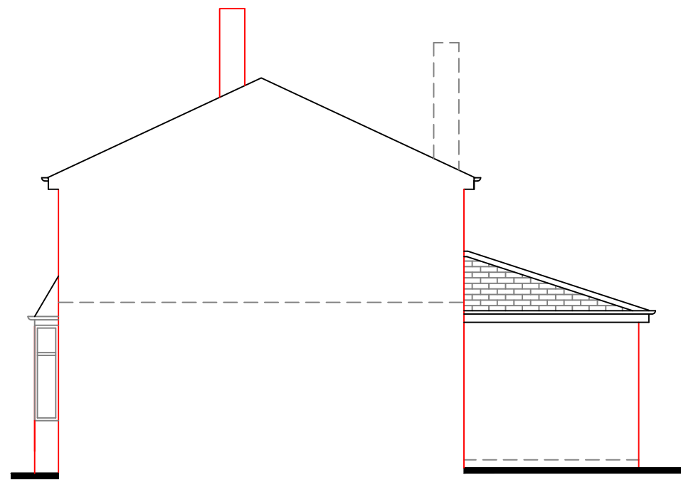
Proposed Shared Boundary Elevation
