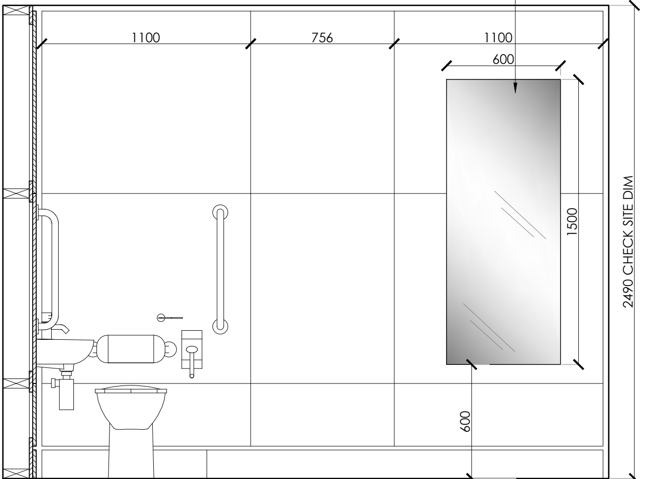
ELEVATION C
