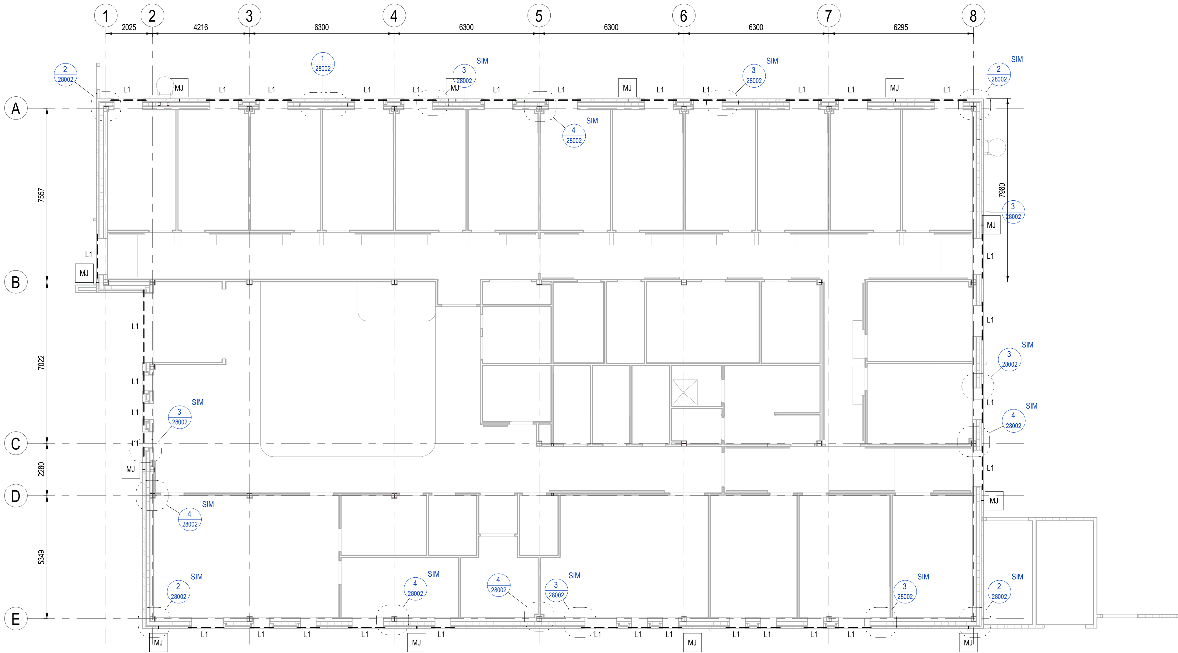
GROUND FLOOR MASONRY GA SCALE: 1 : 100
