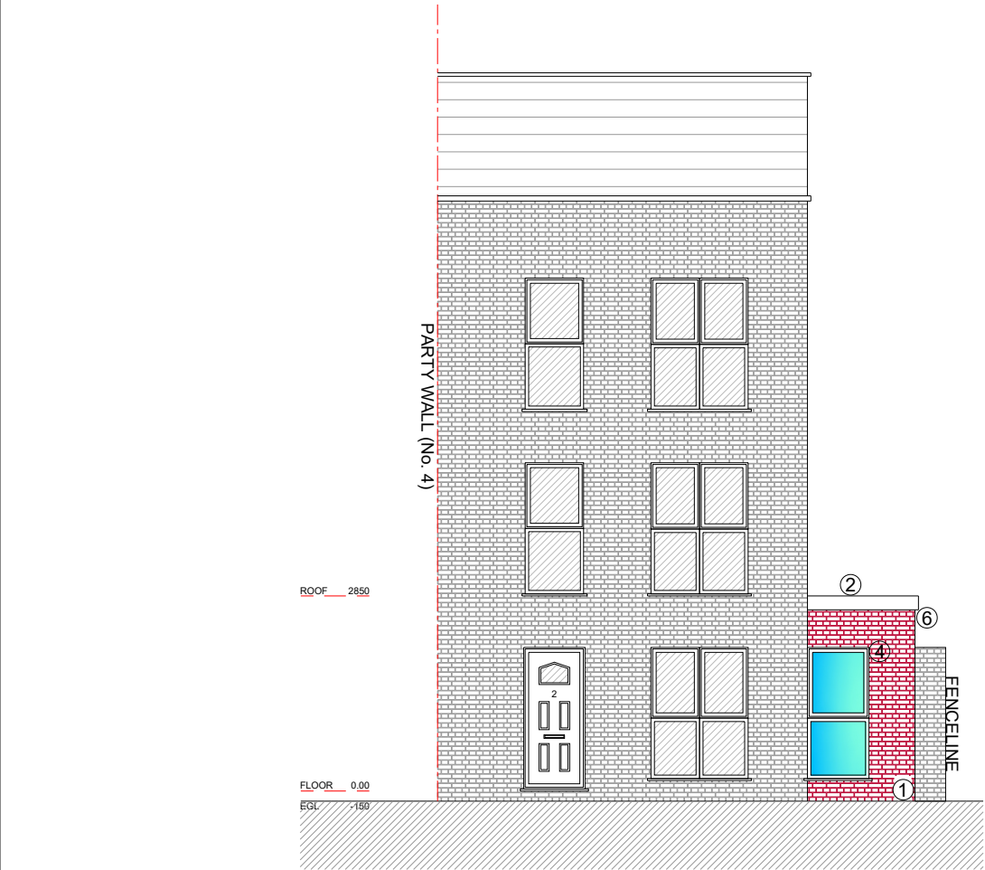
FRONT ELEVATION
