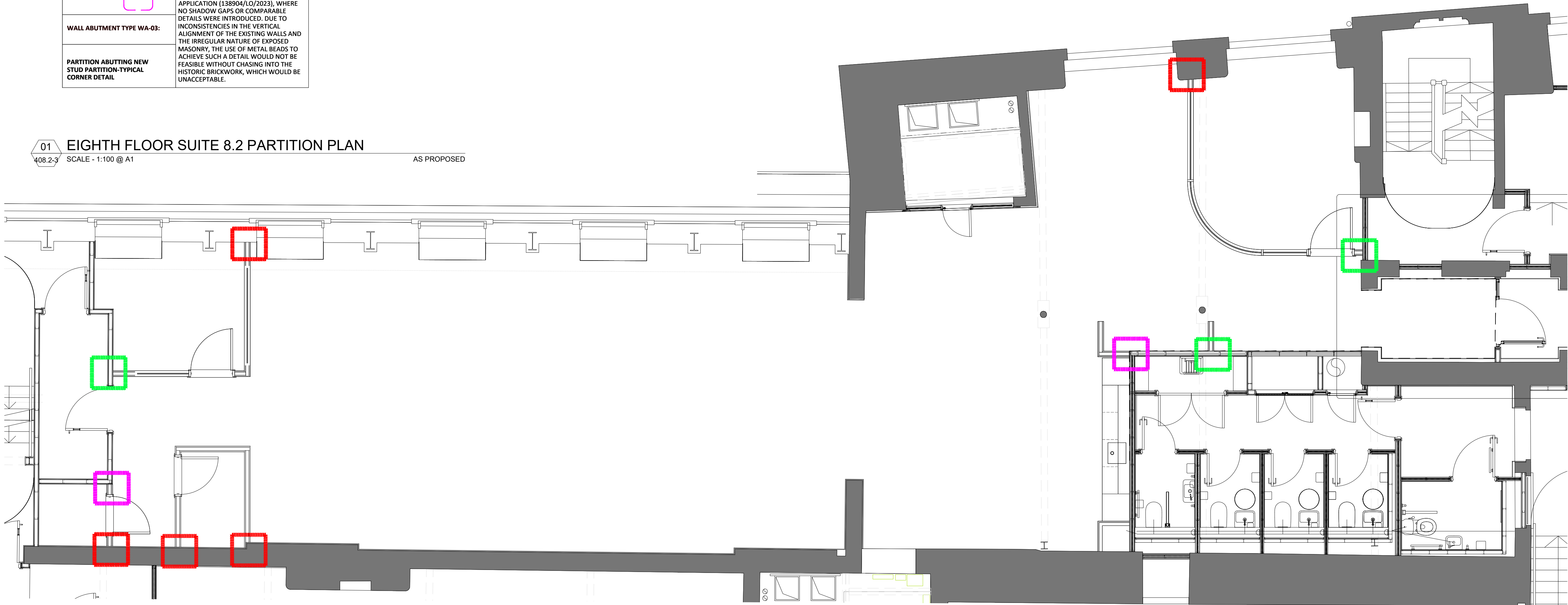
02 EIGHTH FLOOR SUITE 8.2 PARTITION PLAN
