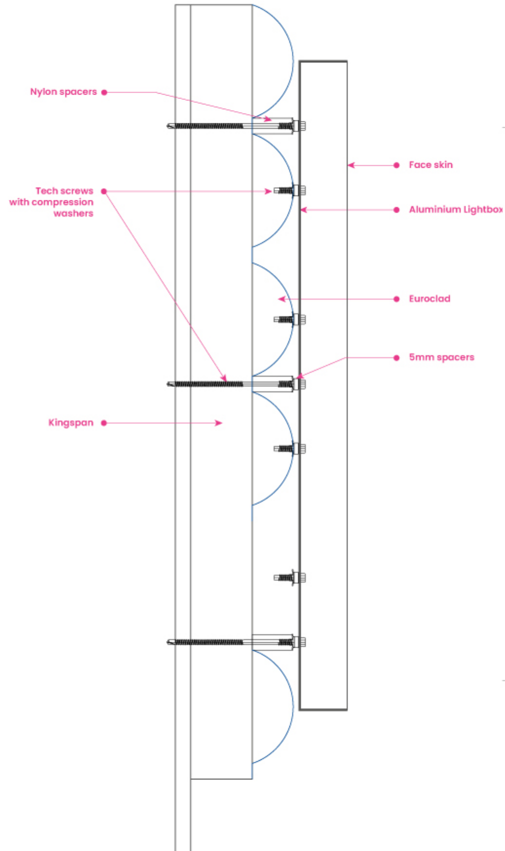
Fixing Detail
