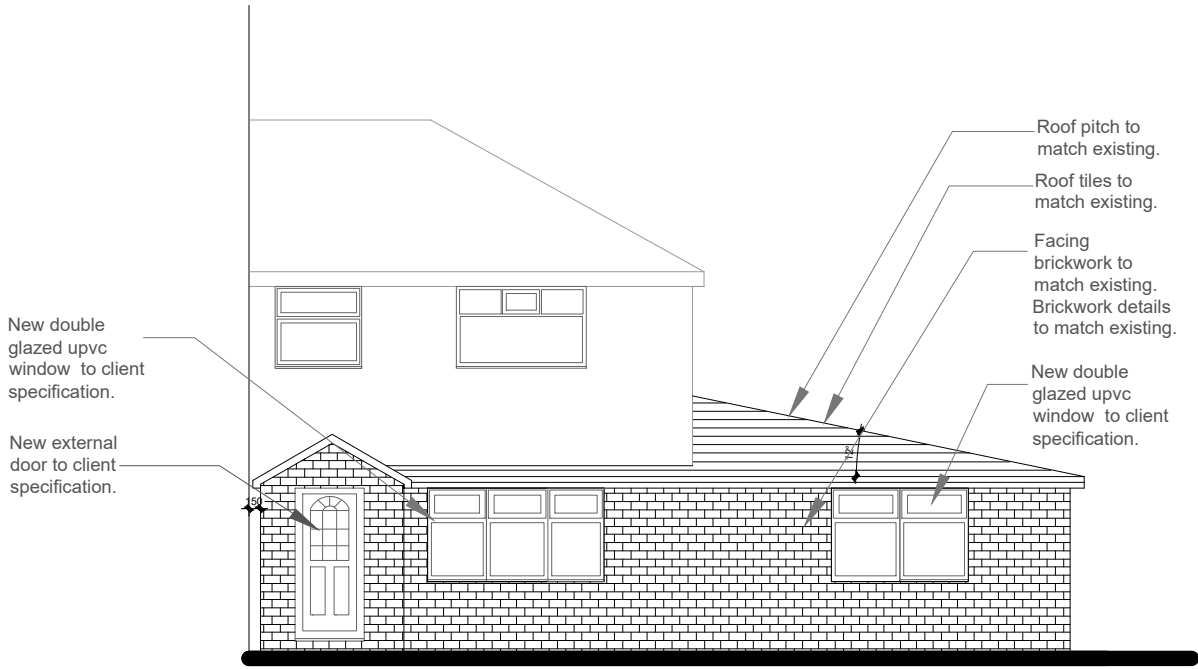
Front Elevation
