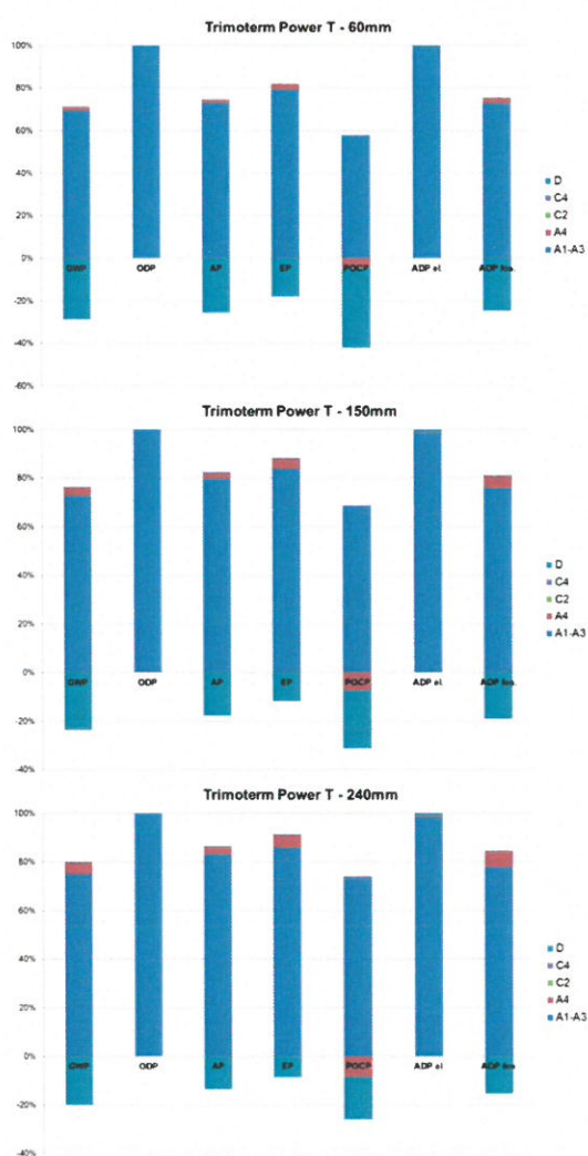
Figure 4: The relative contributions of different life cycle stages (i.e. modules A1-A3, A4, C2, C4 and D) to the environmental impact of Trimoterm Power T façade panels
