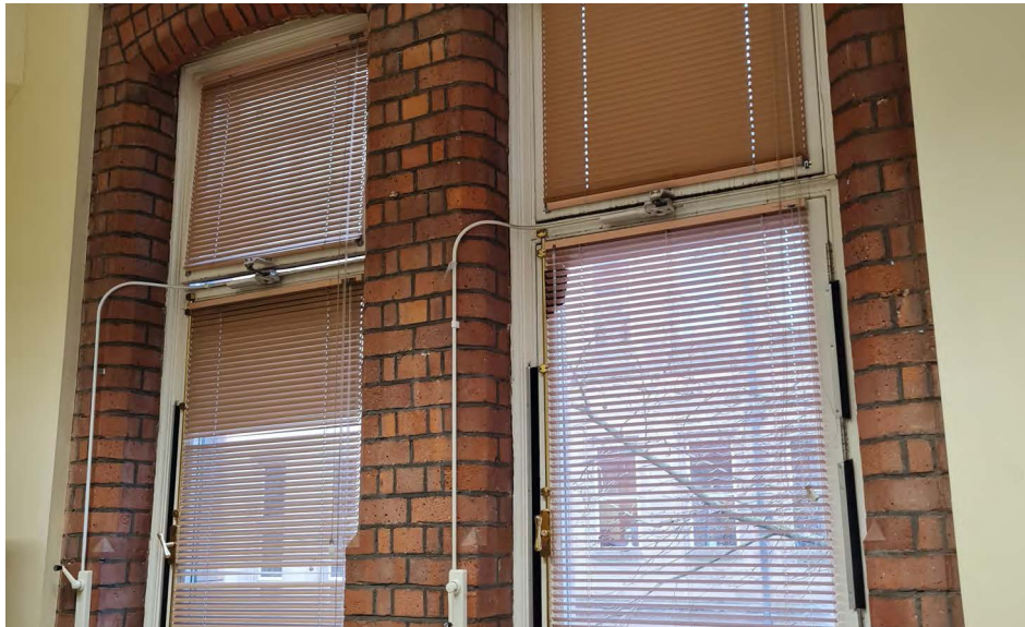
▲ Surface mounted dado trunking, containment and services within cellular spaces
